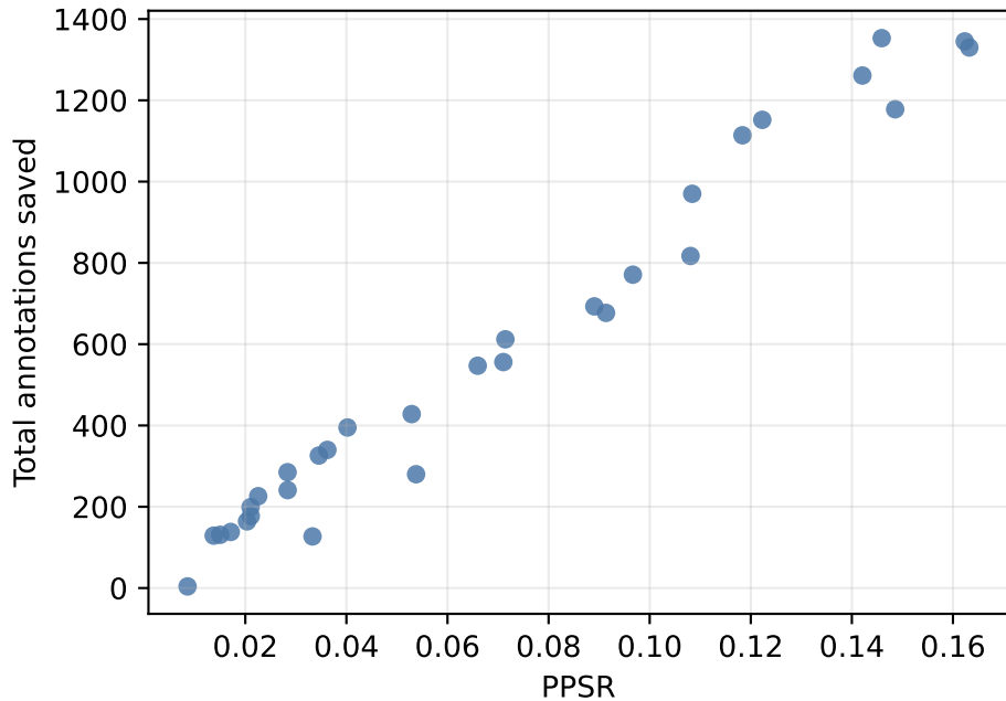
wmt22 en-de
