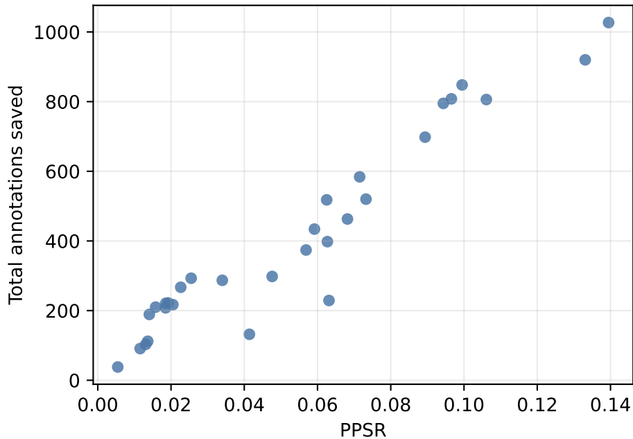
wmt22 en-ru
