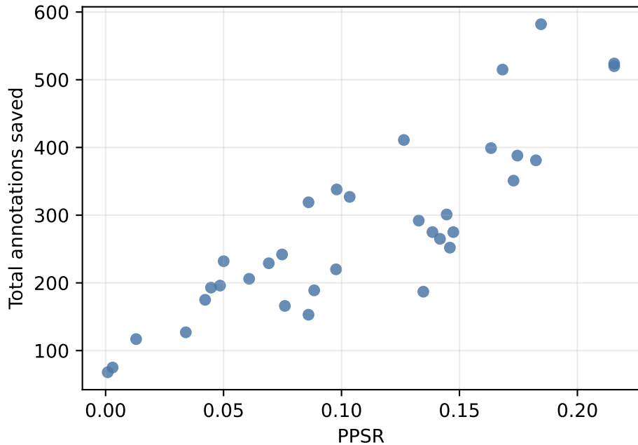
wmt23 en-zh
