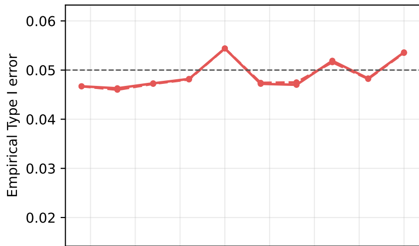
\rho = 0.3, \mathbb{E}[f] = 0
