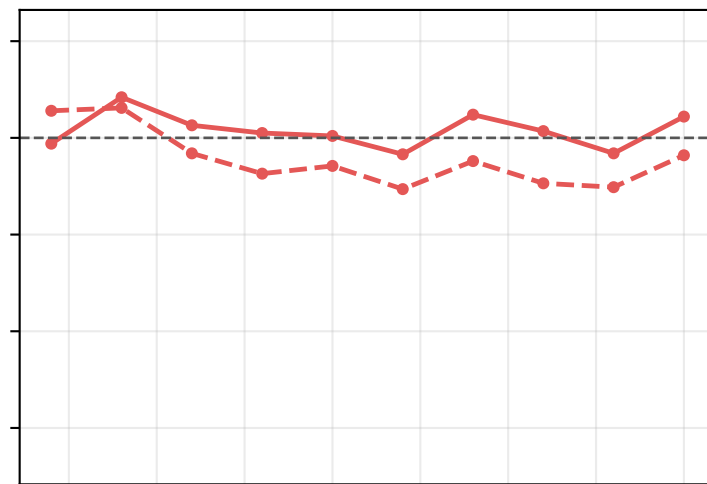
\rho = 0.3, \mathbb{E}[f] = 5
