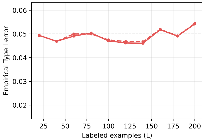
\rho = 0.7, \mathbb{E}[f] = 0
