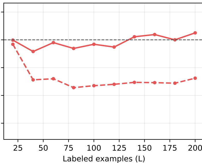
\rho = 0.7, \mathbb{E}[f] = 1
