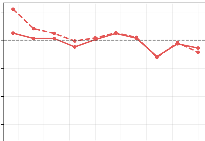
\rho = 0.3, \mathbb{E}[f] = 1
