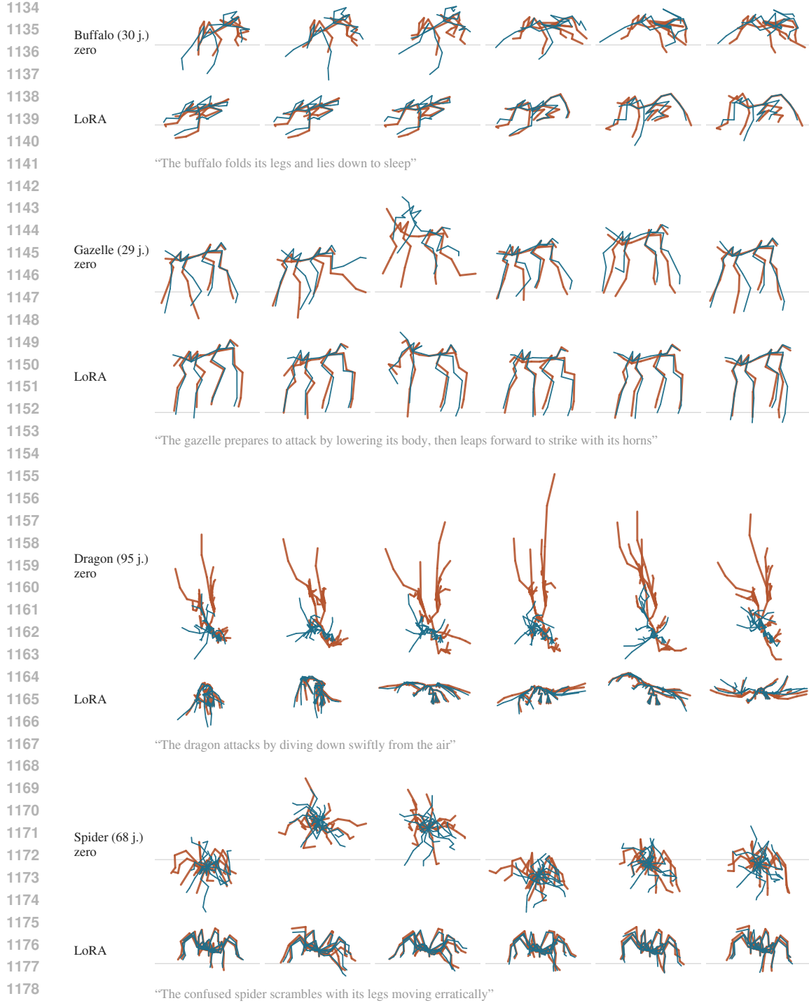
1181 Figure 3: Truebones arms of Table 2: one held-out clip per rig, six frames spread evenly over the 1182 clip, three-quarter view; the quoted sentence is the conditioning prompt. In every panel the directly 1183 predicted joint positions (clay) are overlaid by the forward kinematics of the predicted rotations 1184 (teal); a visible separation is the projected FK-pose discrepancy (a single view can hide a disagree- 1185 ment in depth). Rows: the library model with the rig’s statistics only ( zero , the unadapted snapshot, 1186 whereas the zero column of Table 2 is read after at most 15 warm-up steps) and the per-rig adapter 1187 ( LoRA ). Frames are anchored on the root horizontally and keep their height above the floor; the grey line marks the floor height beneath the root. The Dragon, a flying rig, is anchored on the root in all axes, which removes its dive trajectory. Both rows of a rig are drawn at the same scale.
