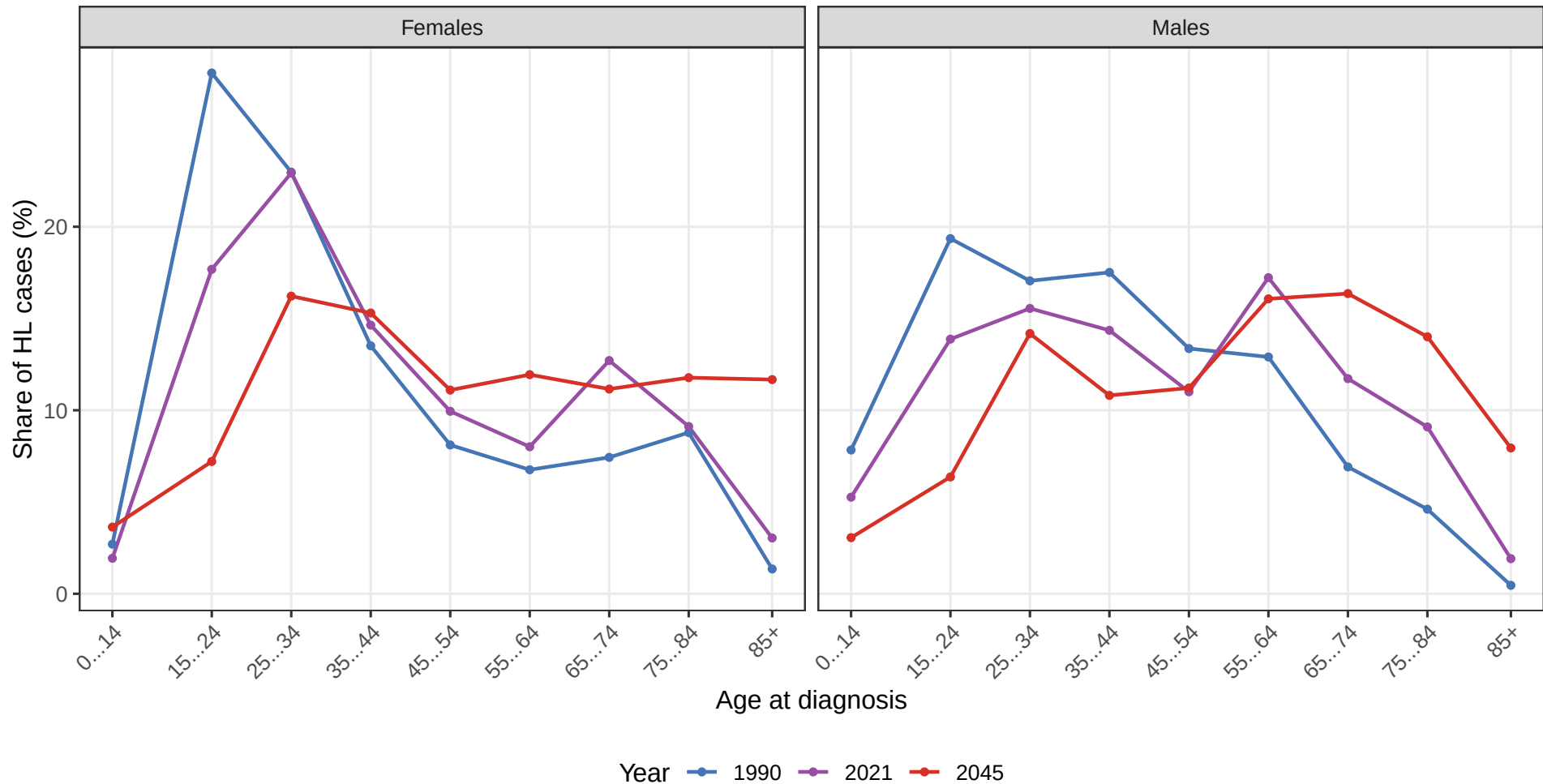
The younger-adult peak shrinks and the older peak grows as cases shift to older ages
