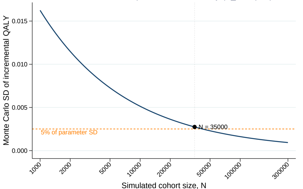
Monte Carlo error vs parameter uncertainty (B_transport)
