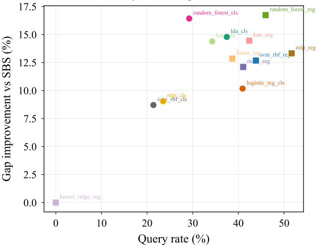
Query rate vs improvement
