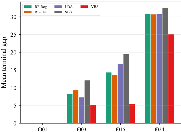
(a) Gap by function
