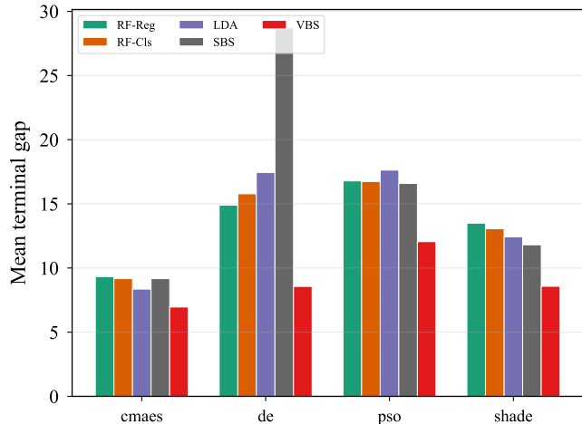
(b) Gap by prefix algorithm
