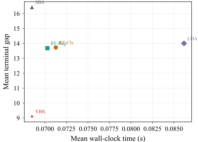
(b) Pareto: gap vs time
