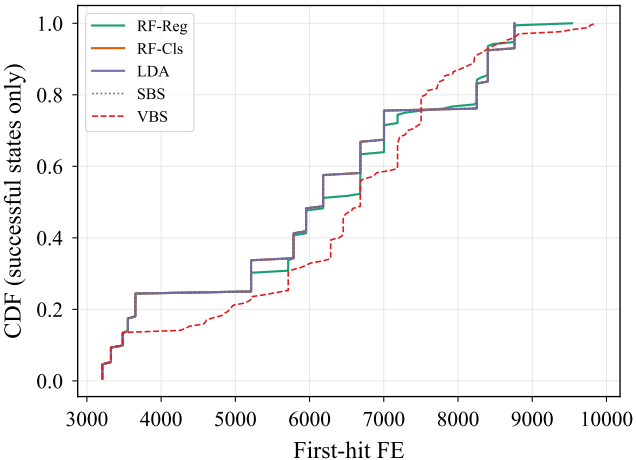
(a) Convergence speed (FE)
