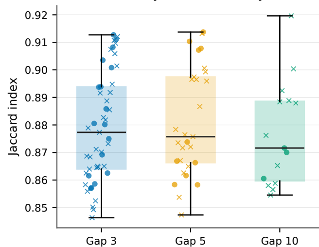
Zero-pattern overlap
