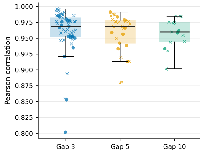
Gene-mean agreement
