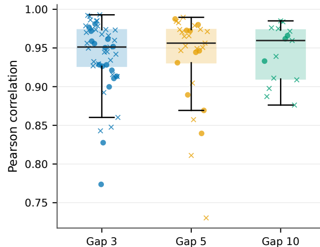
Gene-variance agreement
