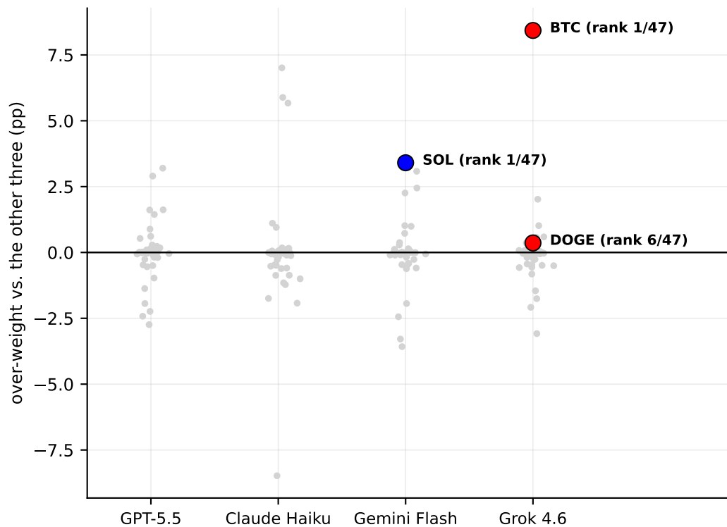
B. All 47 tokens, raw; affiliated assets marked
