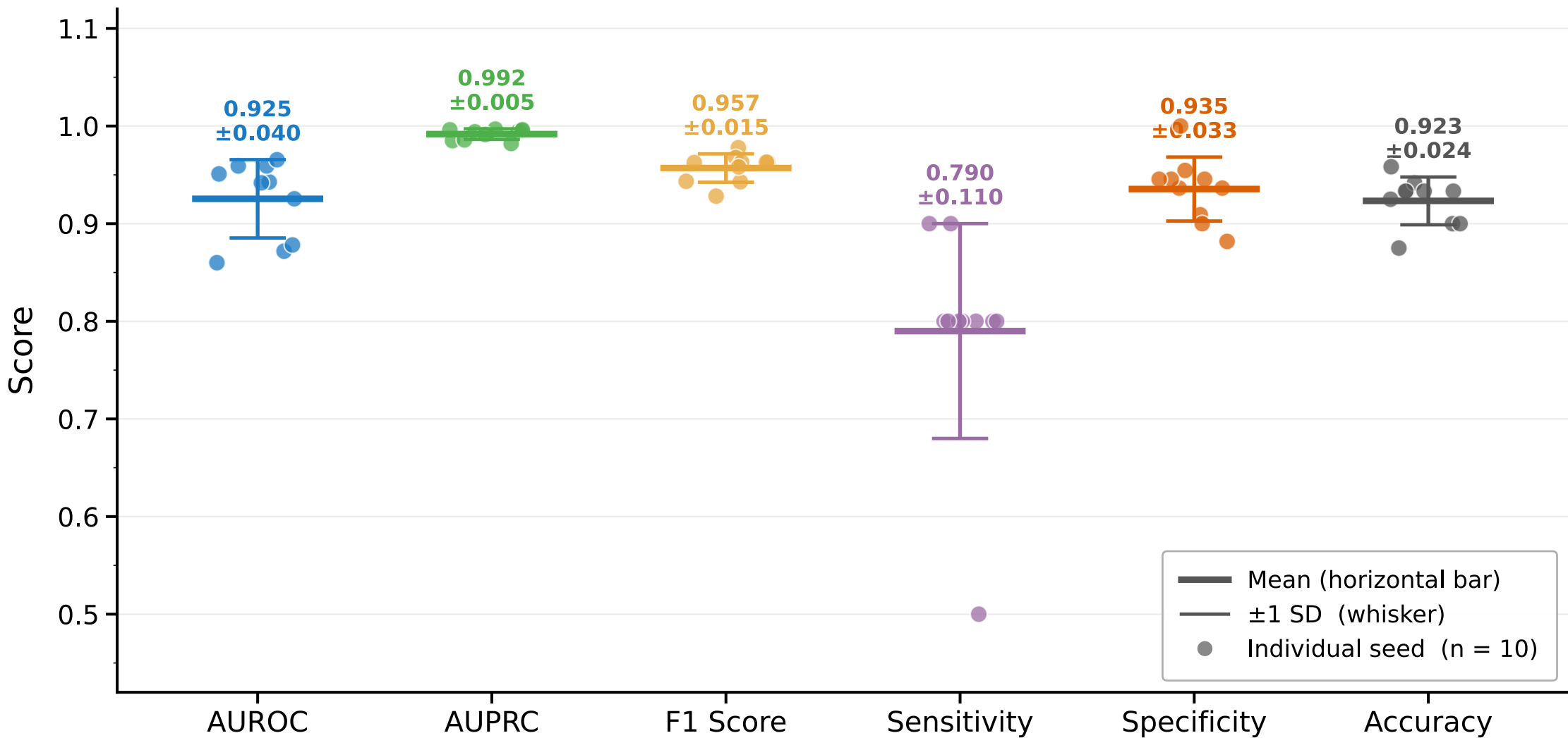
CD-BAN Seed Stability — Performance Across 10 Independent Runs Test Set (n = 120) | Seeds 42-51
