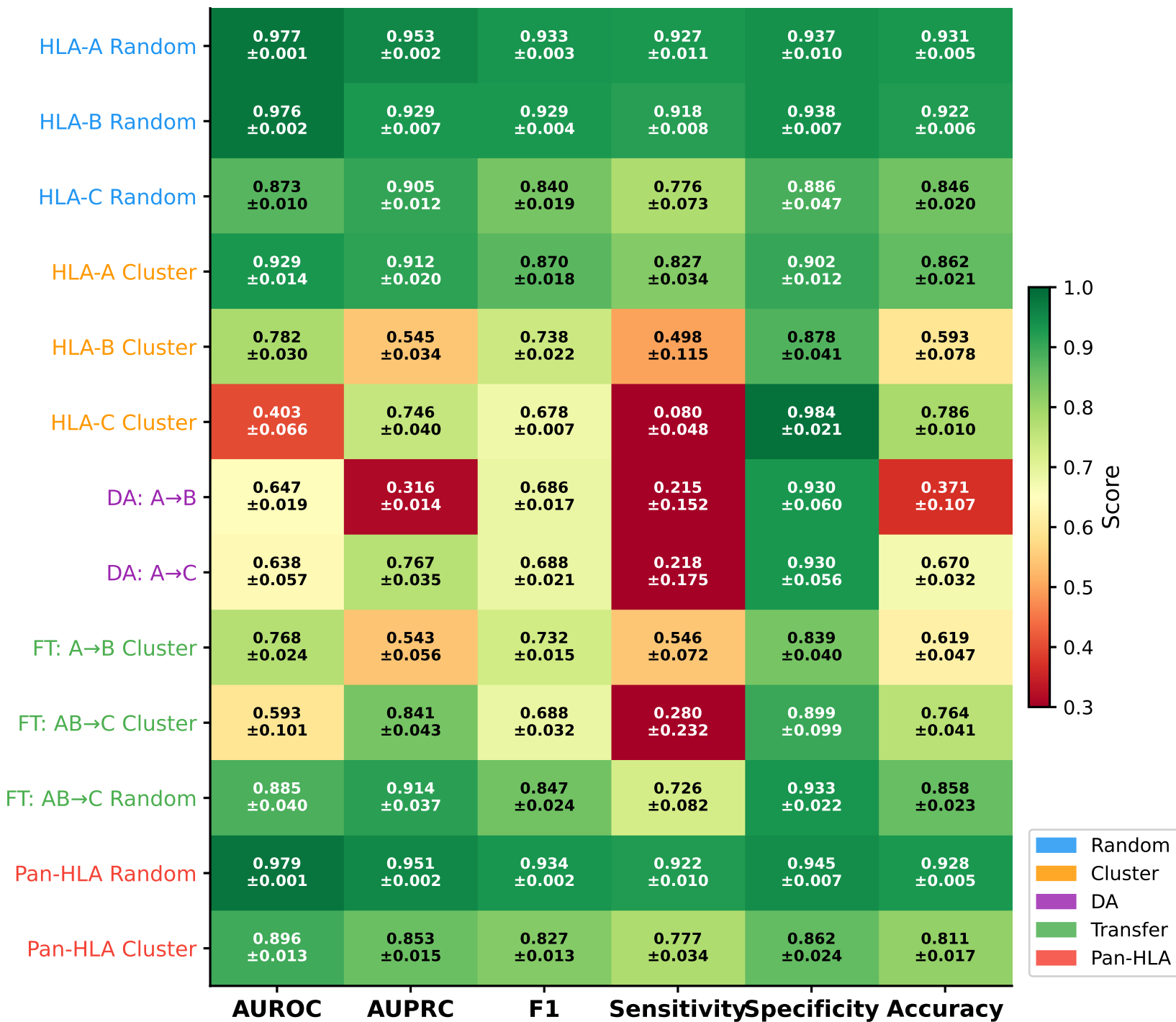
MHCBAN — All Metrics Summary (Mean \pm SD, n = 10 seeds)
