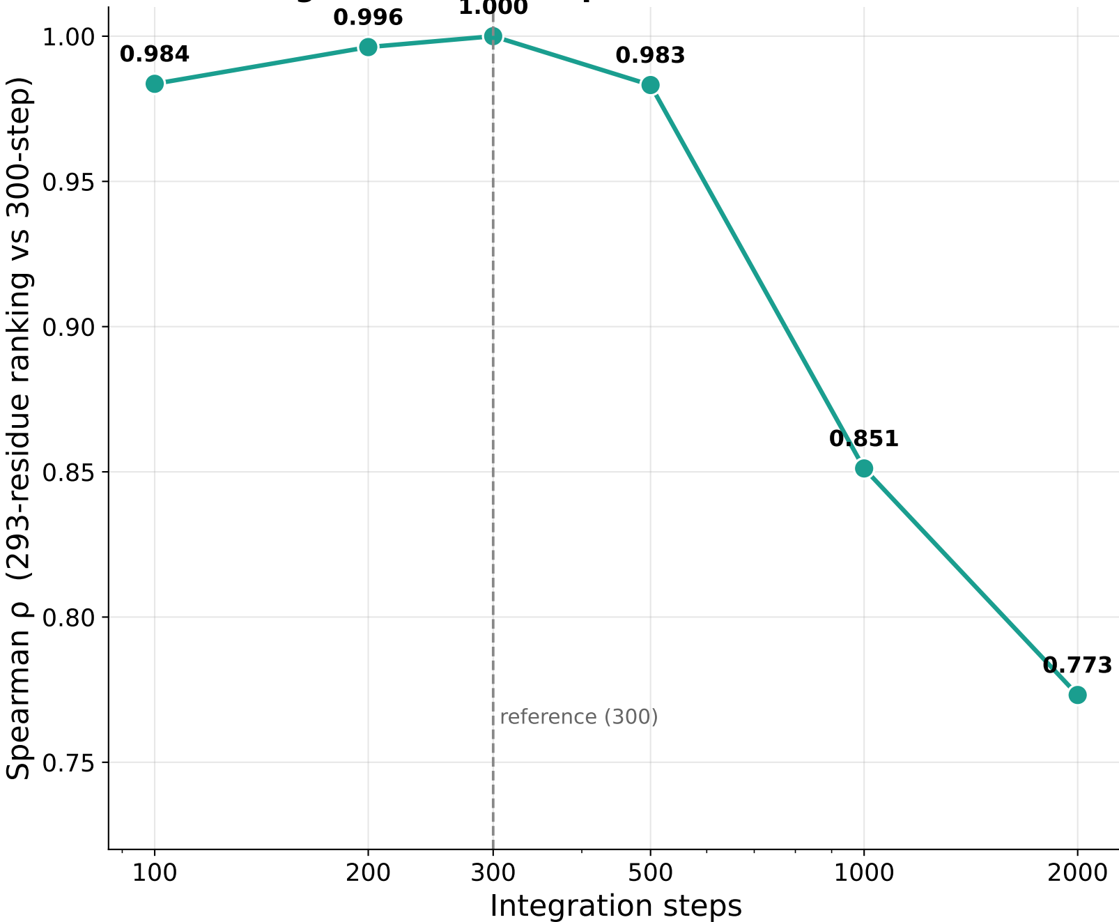
(A) Ranking is robust to step count
