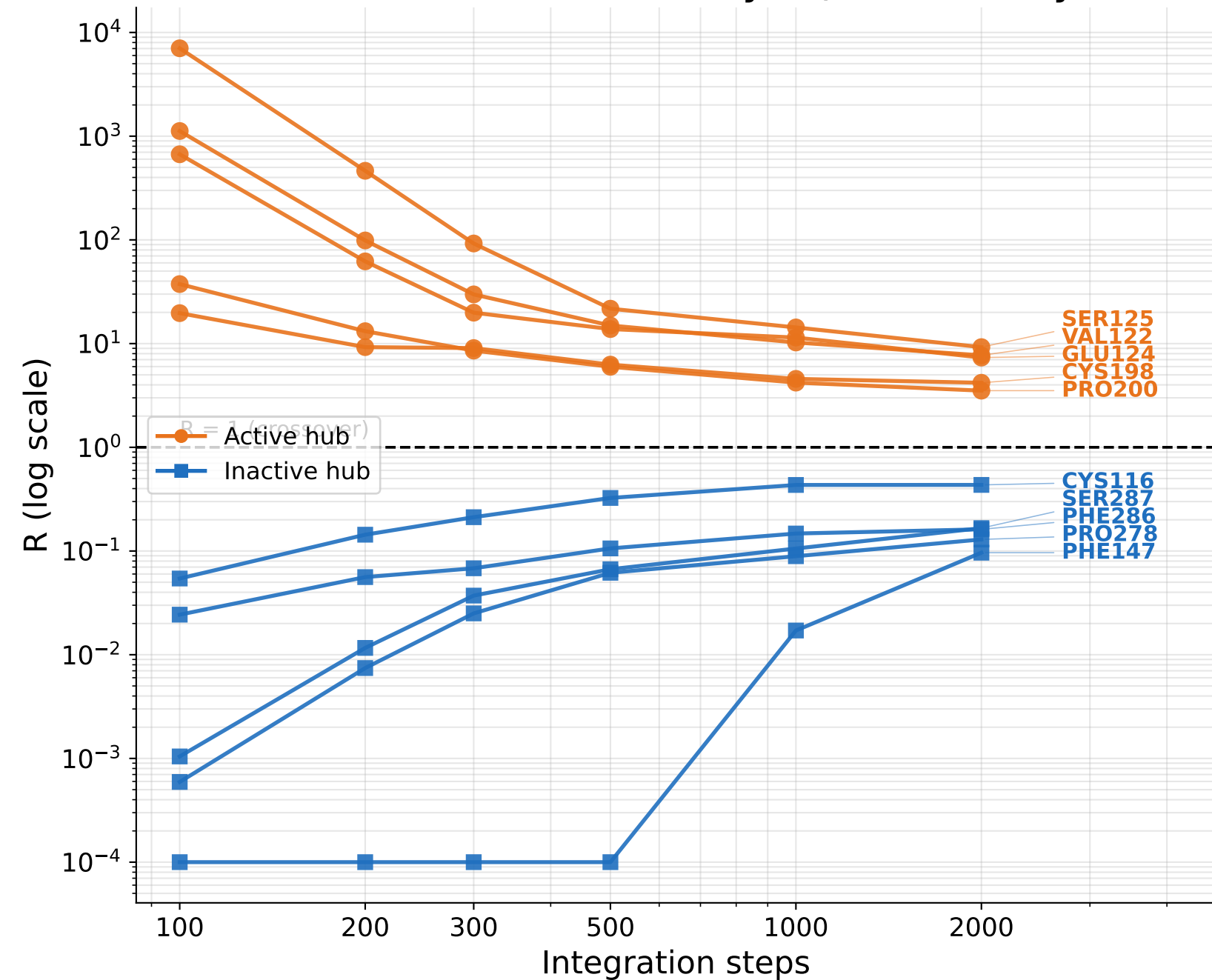
(B) Direction is robust: Active stay >1, Inactive stay <1
