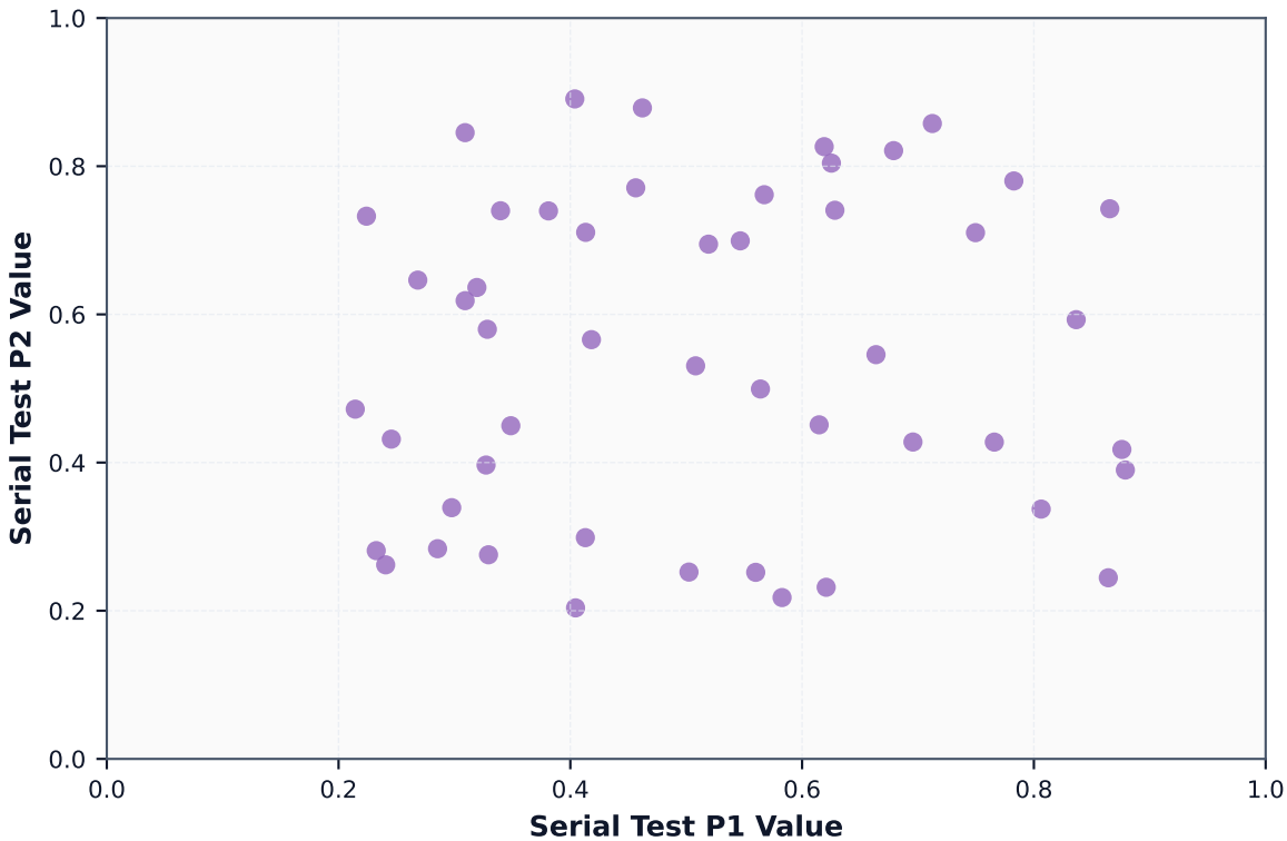
NIST Serial Test Dual P-Value Correlation (P1 vs P2)
