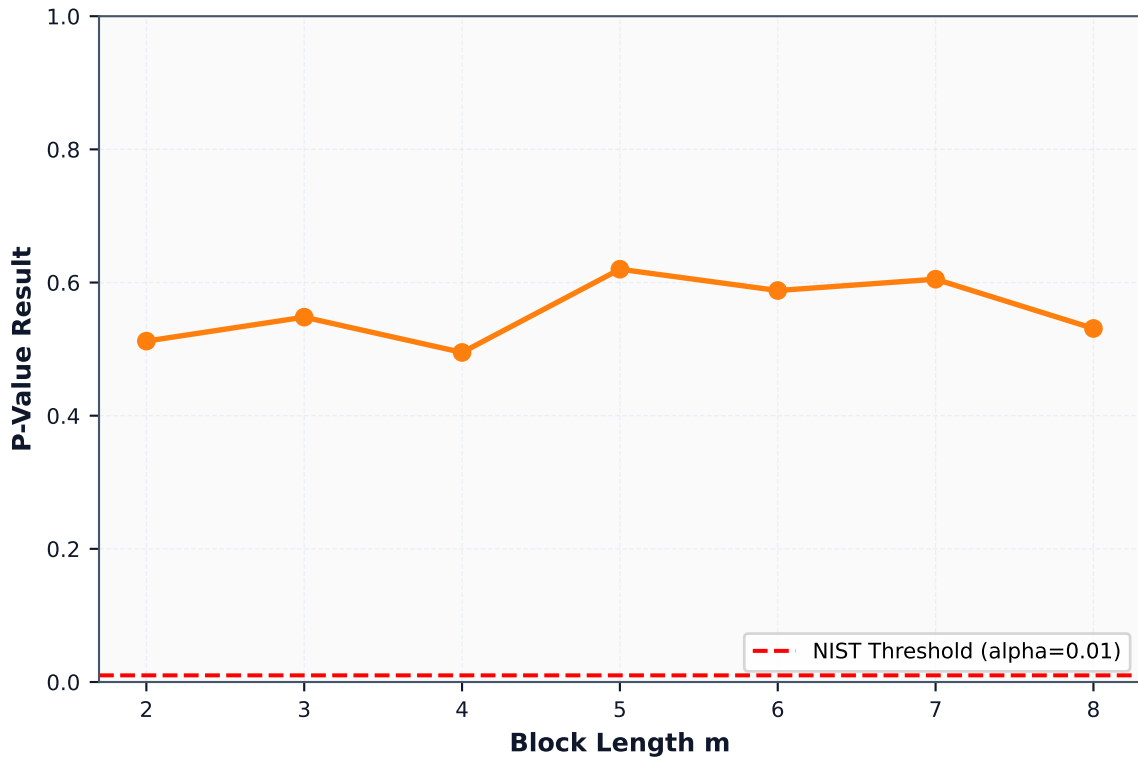
NIST Approximate Entropy Test vs Block Length m
