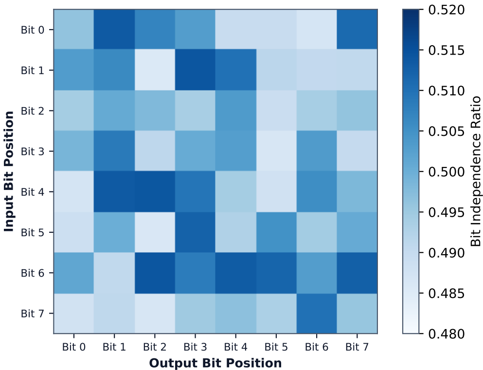
Bit Independence Criterion (BIC) Matrix
