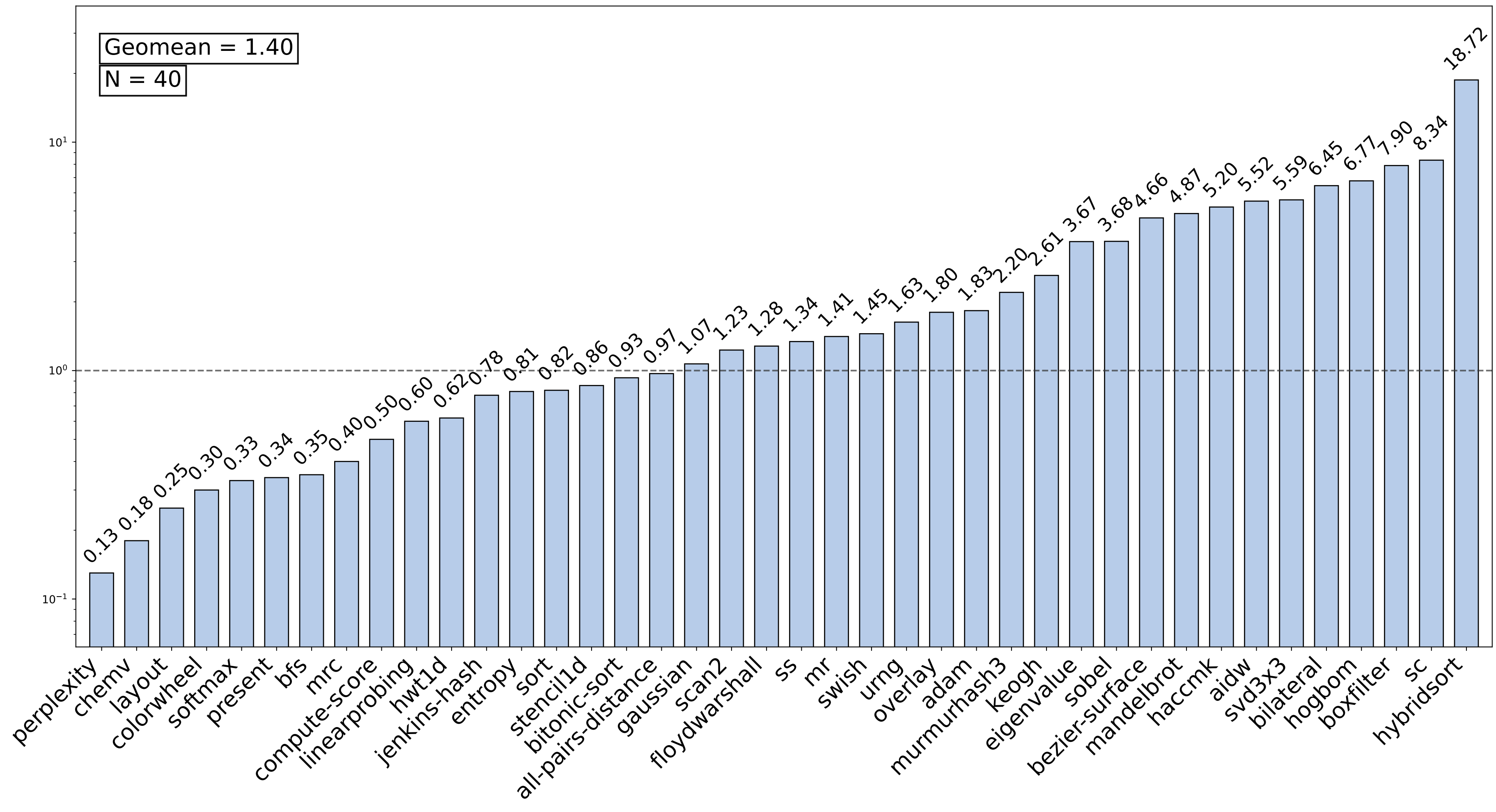
ARM chipStar-v1.2.1 GPUOCL speedup over CPU PoCL
