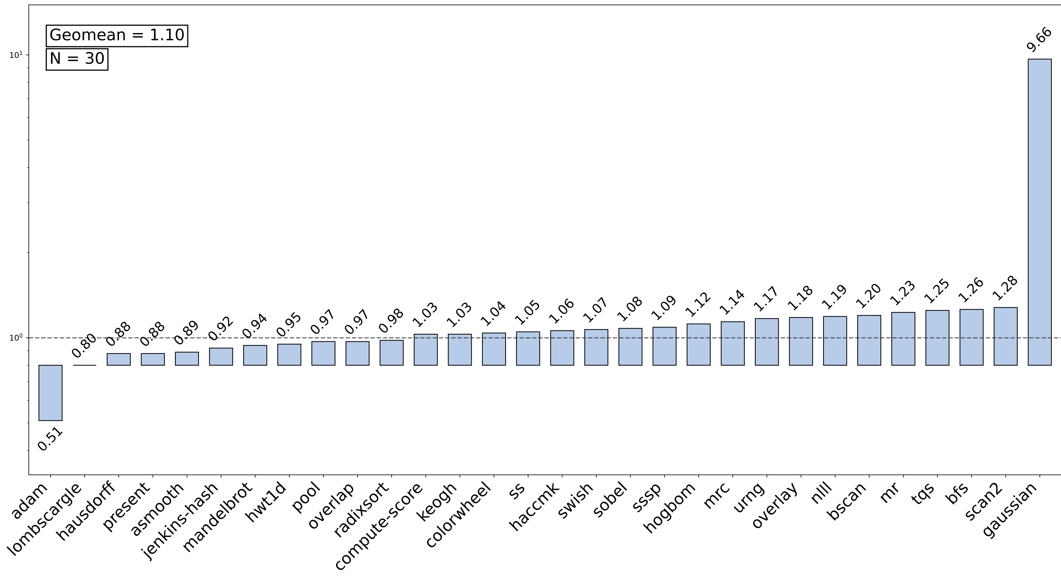
Arc770 chipStar-v1.2.1+JITopt speedup over SYCL(-fp-model=fast)+JITopt (excluding near-equal performance)
