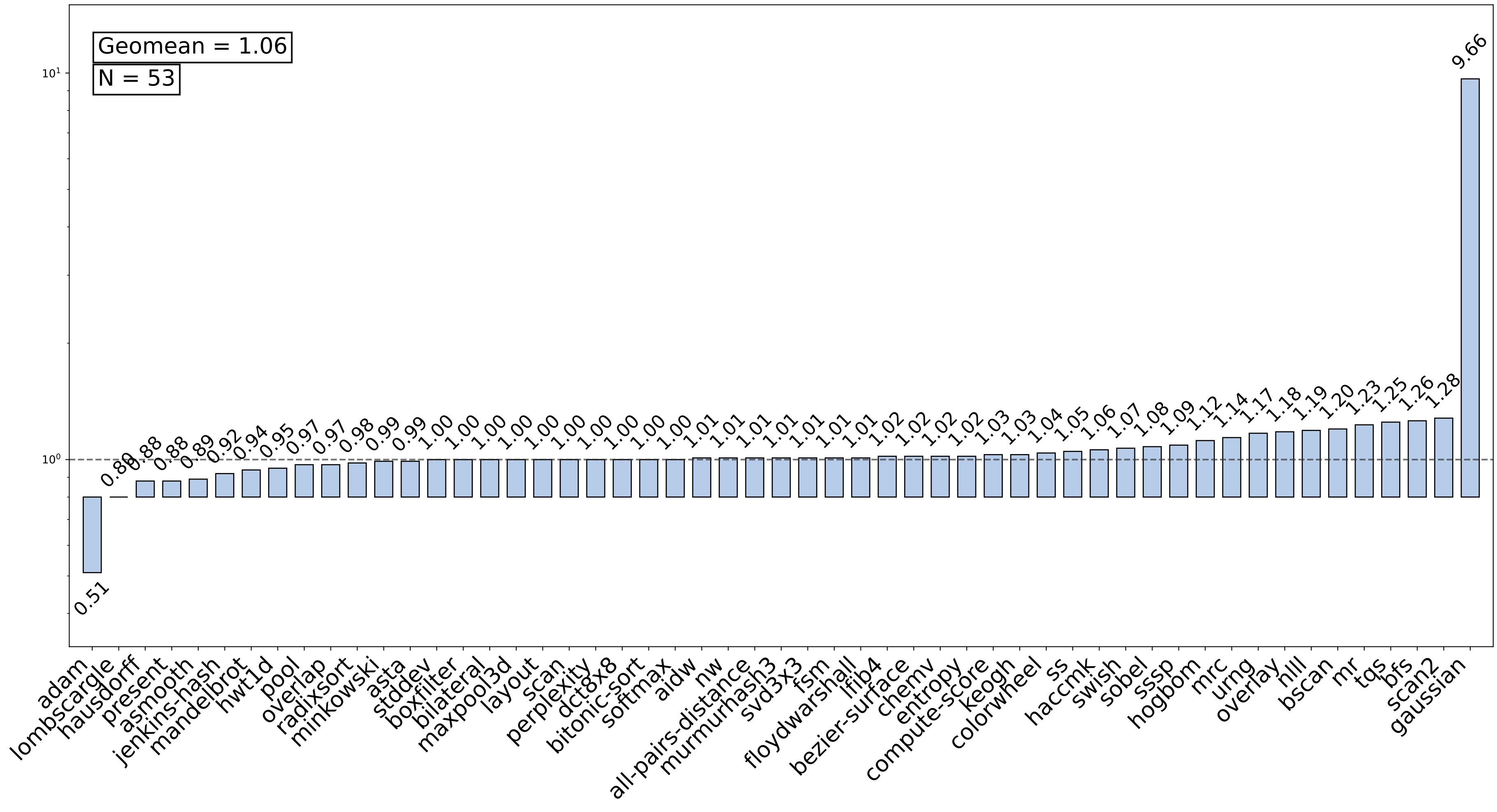
Arc770 chipStar-v1.2.1+JITopt speedup over SYCL(-fp-model=fast)+JITopt
