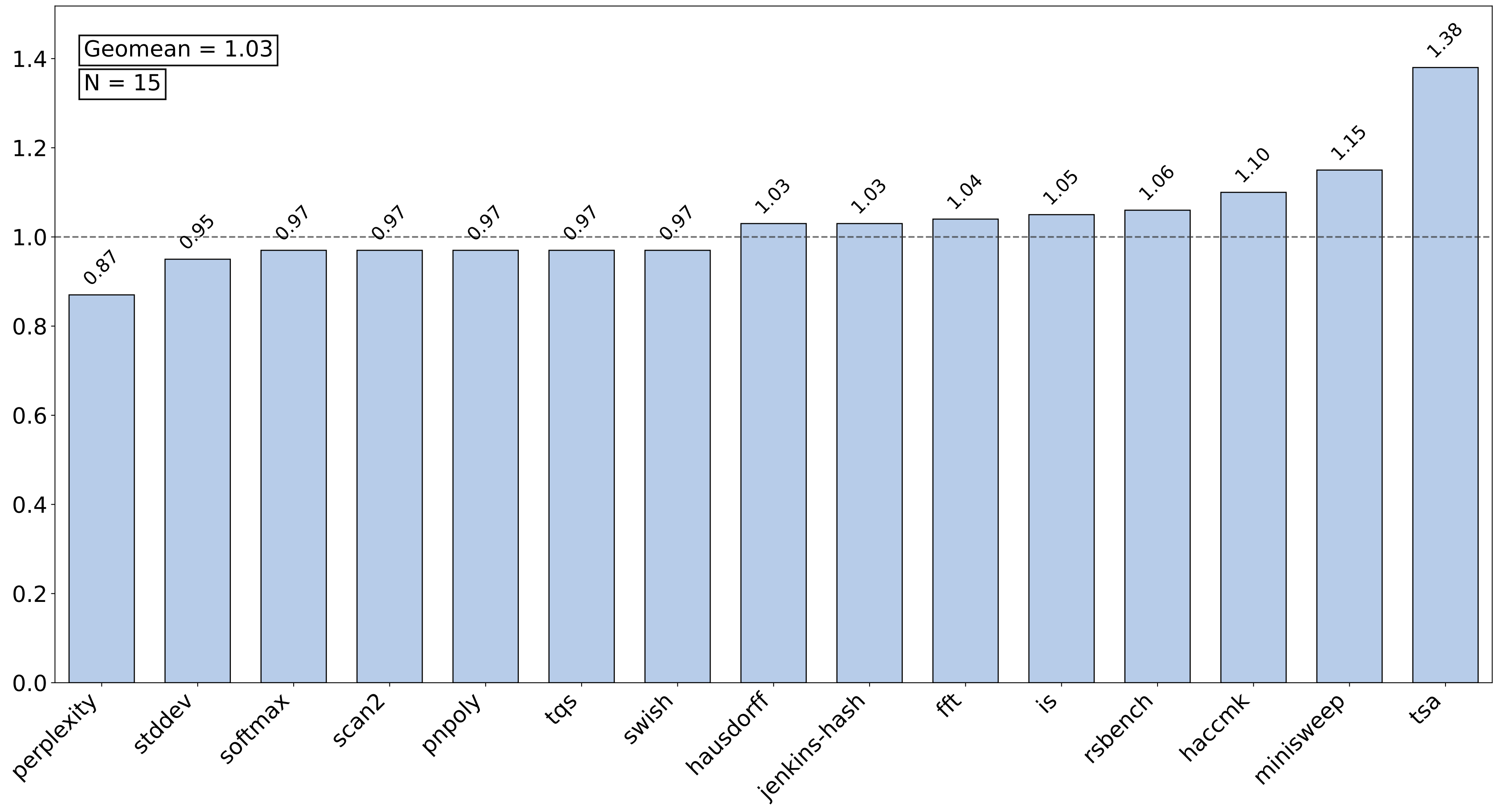
HeCBench, RTX 3060, CUDA SDK vs. rusticl/zink (excluding near-equal performance)
