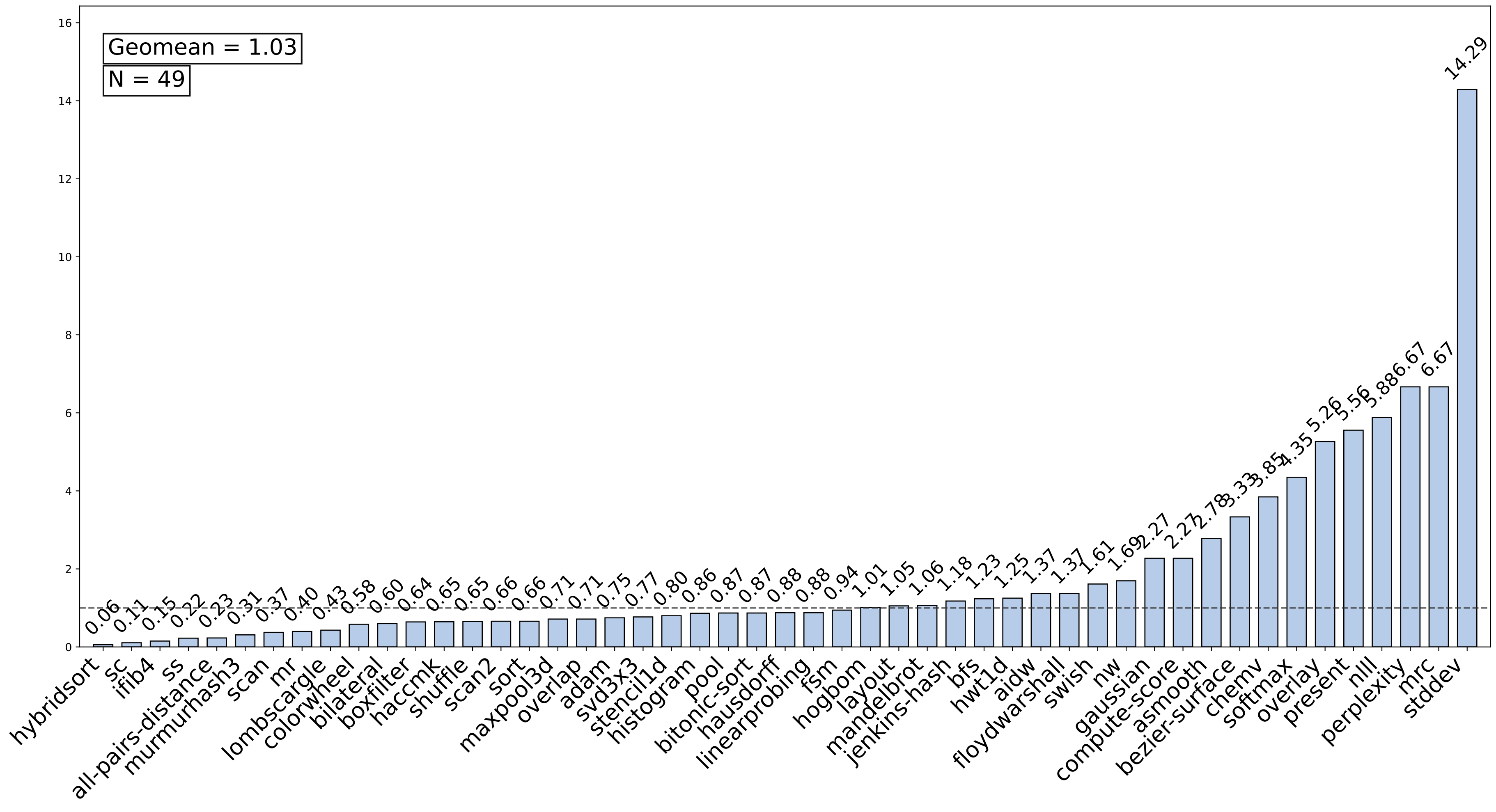
Intel UHD 770 chipStar-v1.2.1(OCL) speedup over OpenCL-CPU
