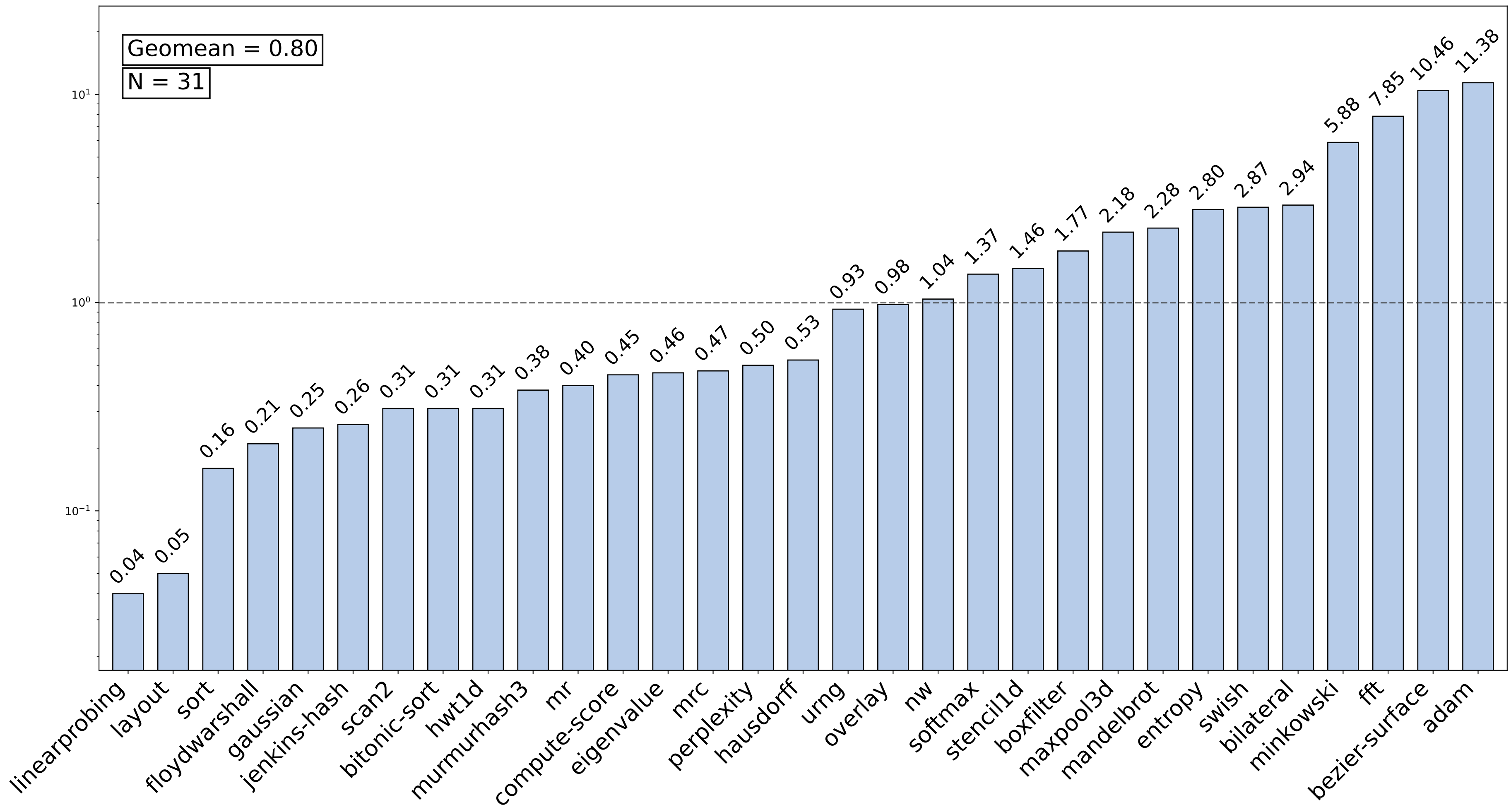
PowerVR BXE-4-32G GPU speedup vs StarFive JH7110 CPU
