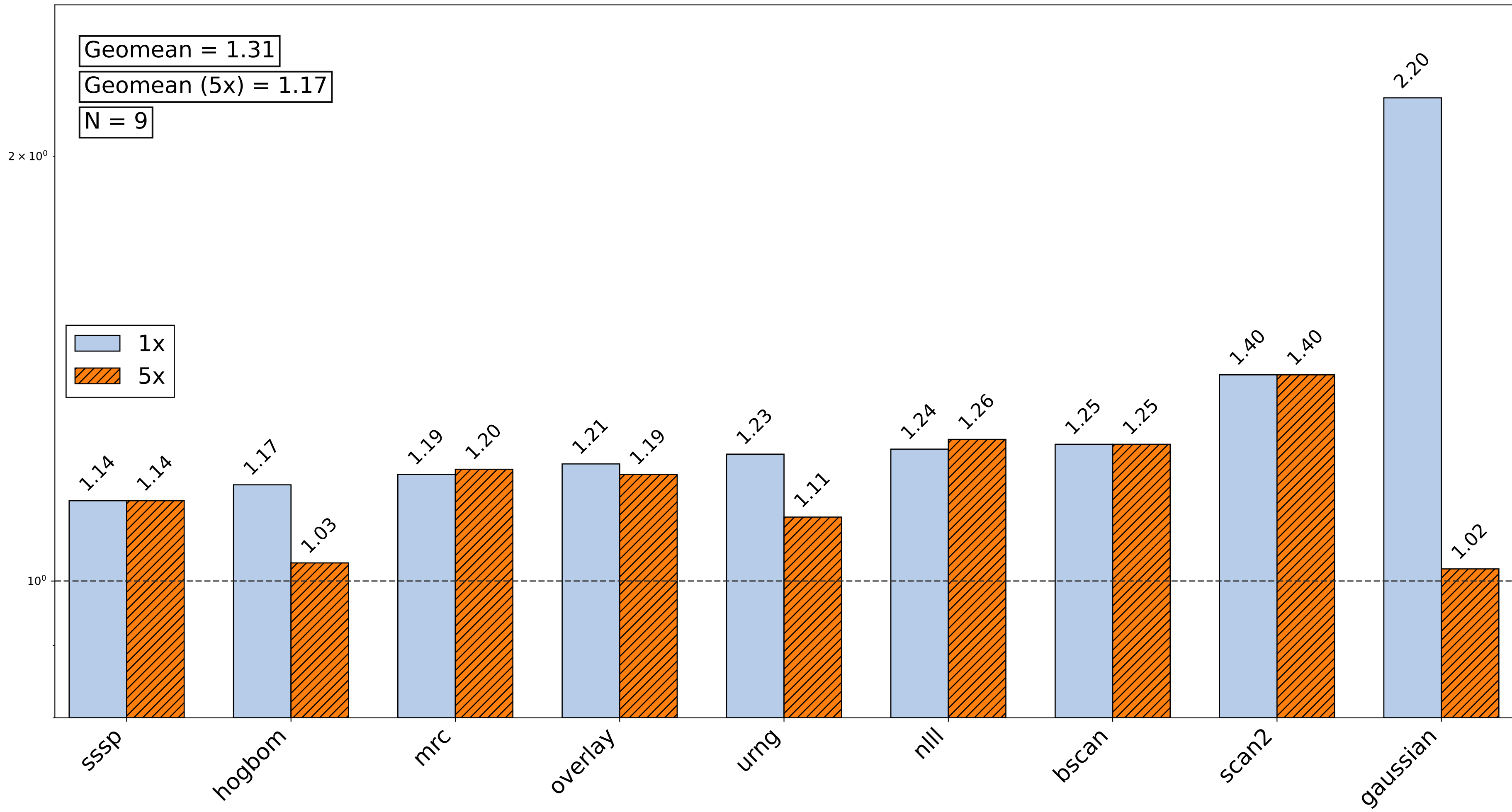
Arc 770 chipStar-v1.2.1 speedup over SYCL, scaling wallclock time
