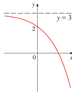
(c) y = 3 - 2^x
