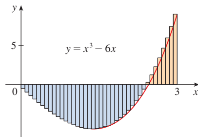
FIGURA 7 R_{40} \approx -6.3998
