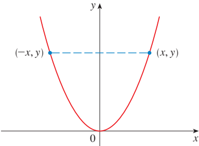
(a) y = ax^2, a > 0
