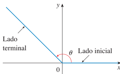
FIGURA 3 \theta \geq 0
