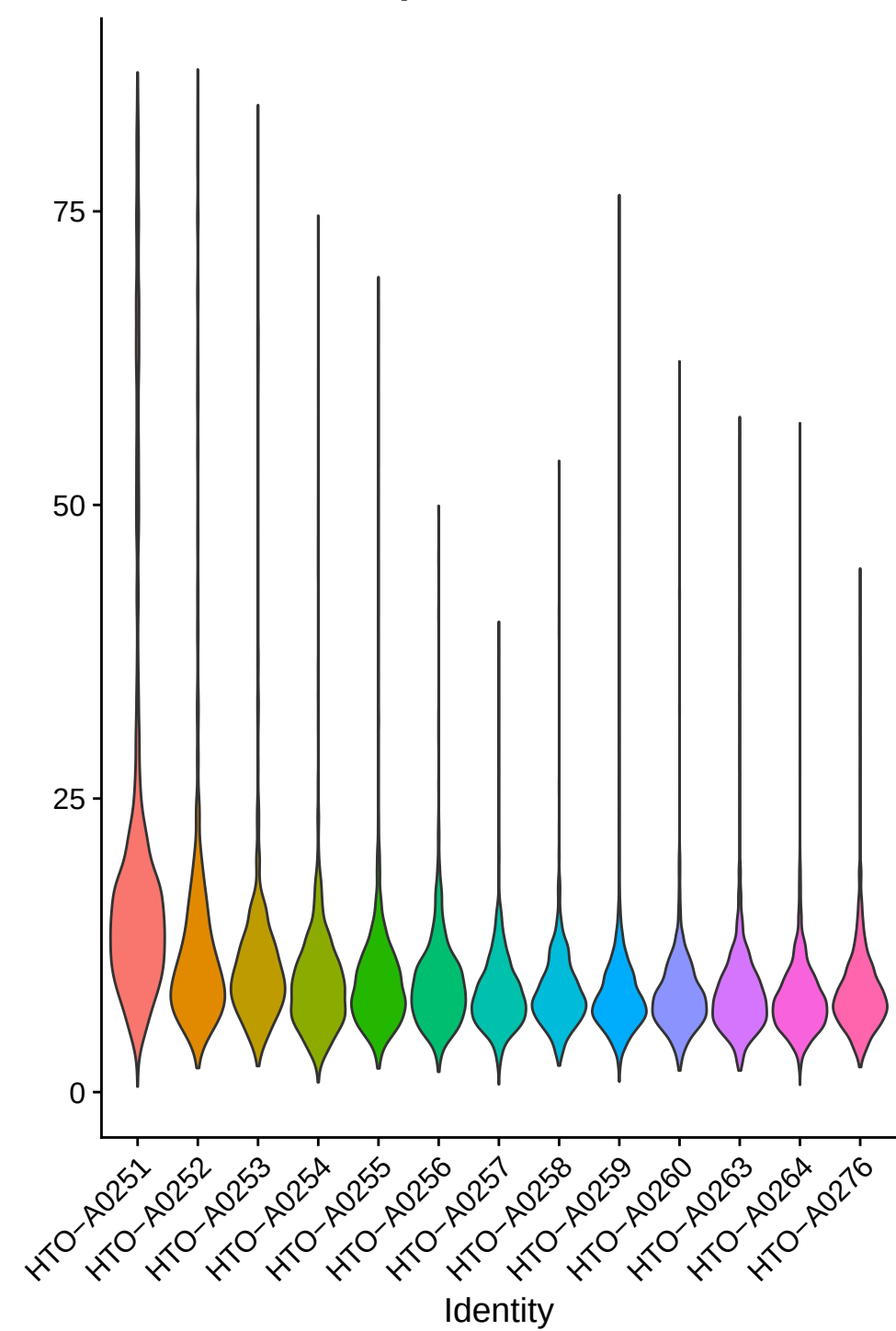
percent.mt
