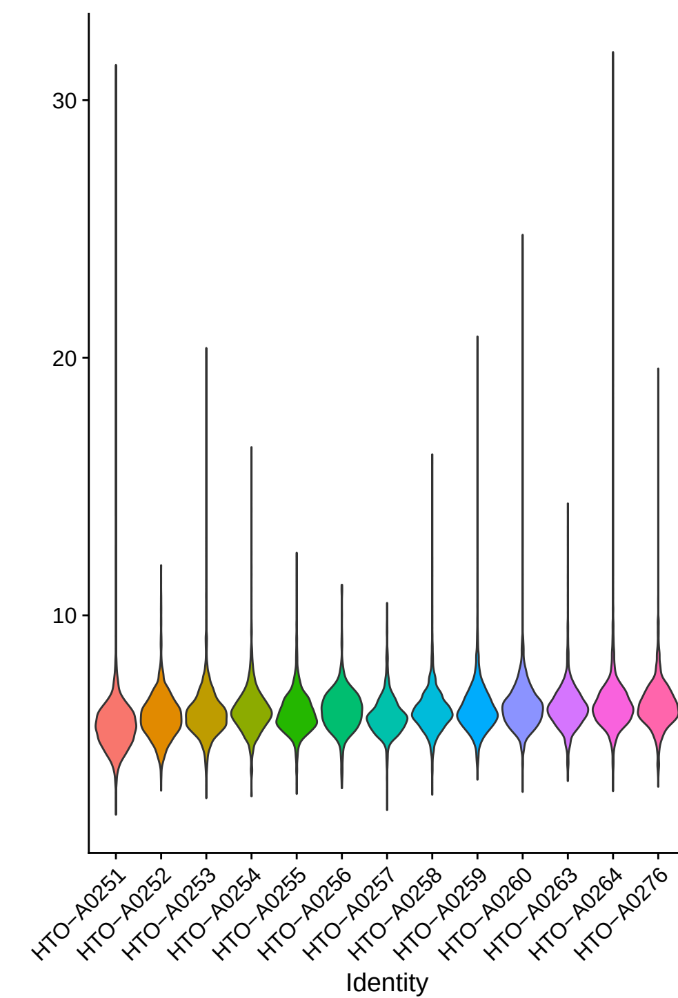
TSS.enrichment
