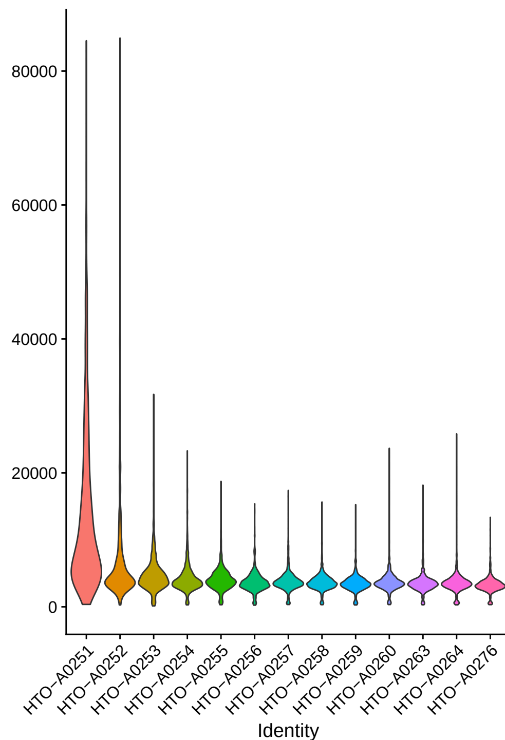
TSS.enrichment
