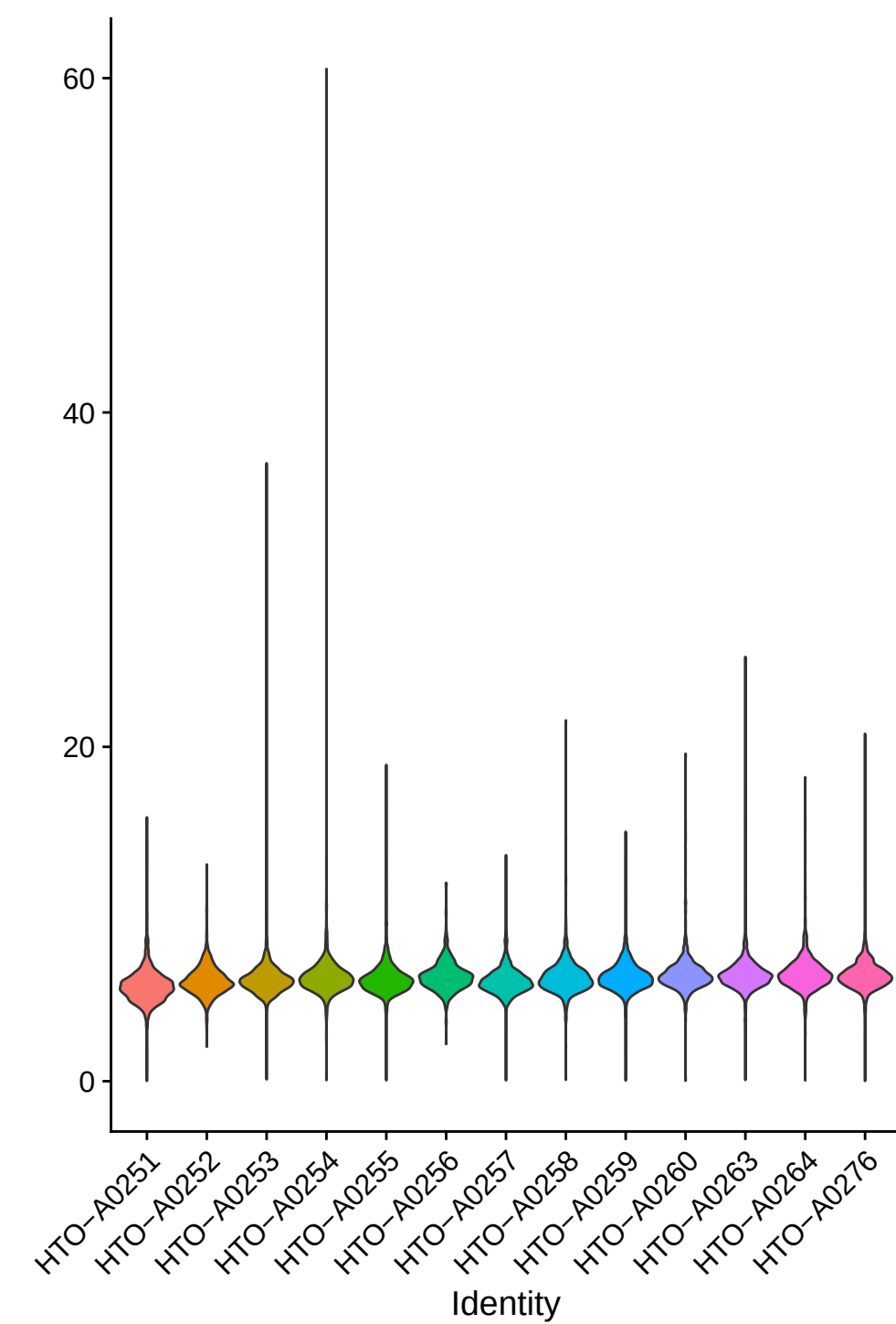
TSS.enrichment
