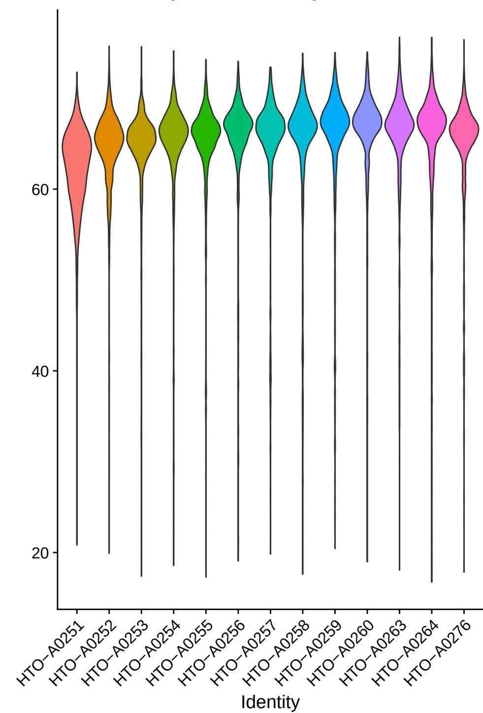
pct_reads_in_peaks
