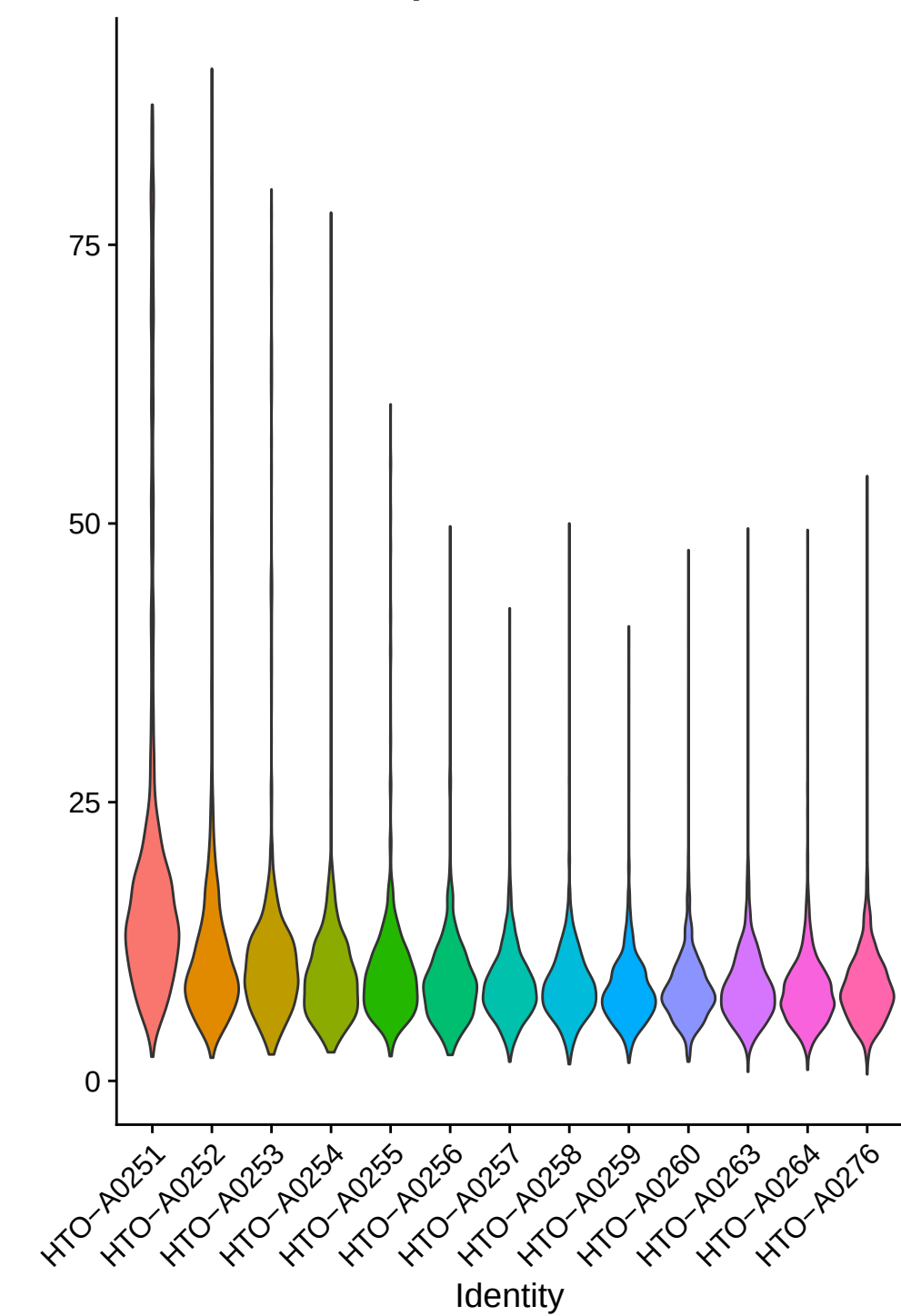
percent.mt
