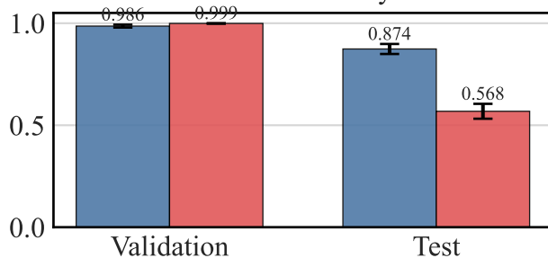
Word Accuracy
