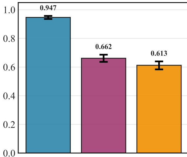
1 - CER
