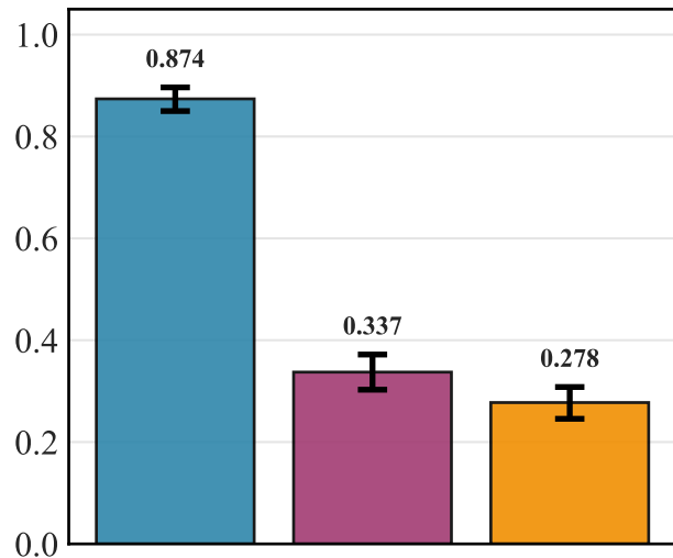
Word Accuracy
