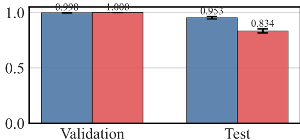
1 - CER
