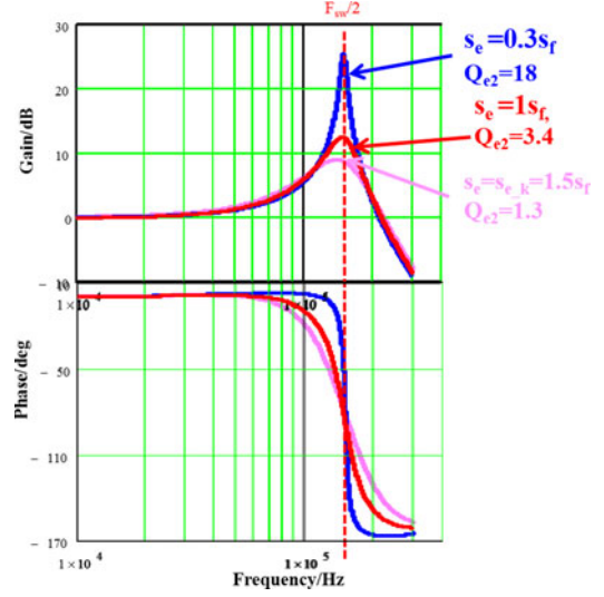
Fig. 5. Bode plots comparison of control-to-output transfer function in region I.
