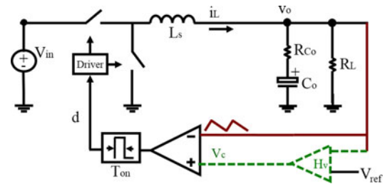
Fig. 1. Structure of constant on-time V^2 control.
