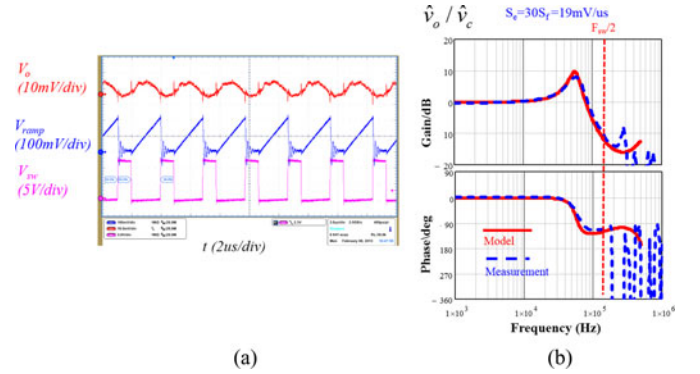
Fig. 19. (a) Steady-state waveform. (b) Small-signal control-to-output transfer function with S_e = 30S_f = 19 \text{ mV}/\mu\text{s} .
