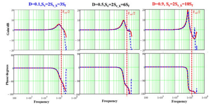
Fig. 14. Bode plots of control-to-output transfer function between model and simulation for different duty cycles: Solid line—Model; Dashed line—SIMPLIS simulation.
