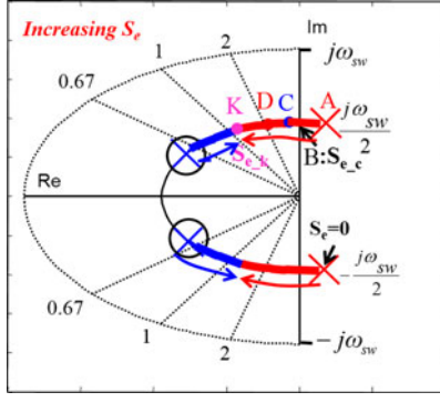
Fig. 4. Pole-zero map of control-to-output transfer function with increasing s_e in region I.
