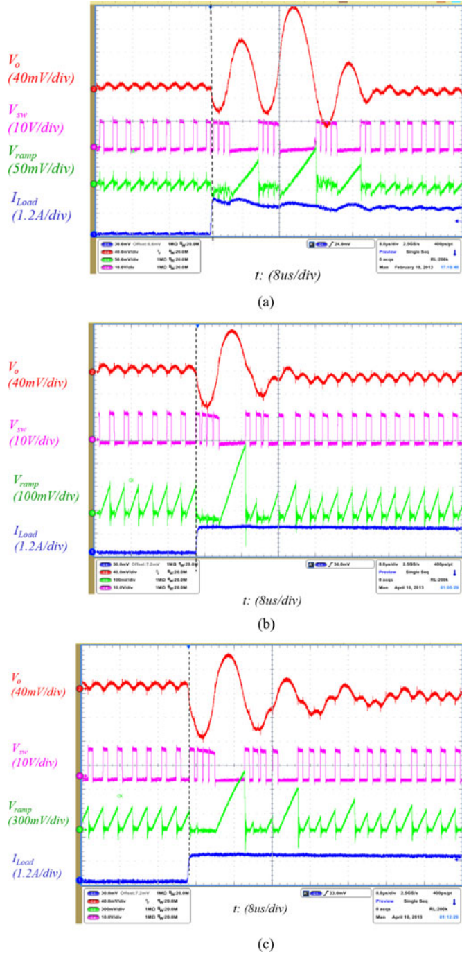
Fig. 20. Load step-up transient performance comparison for 0.5–2 A load step. (a) S_e = 3.5S_f = 2.2 \text{ mV}/\mu\text{s} . (b) Worst case for S_e = 10S_f = 6.3 \text{ mV}/\mu\text{s} . (c) Worst case for S_e = 30S_f = 19 \text{ mV}/\mu\text{s} .
