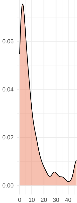
glyphosates
