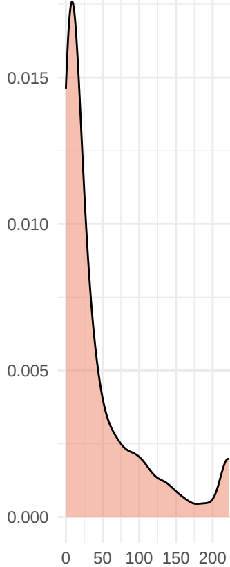
glyphosates
