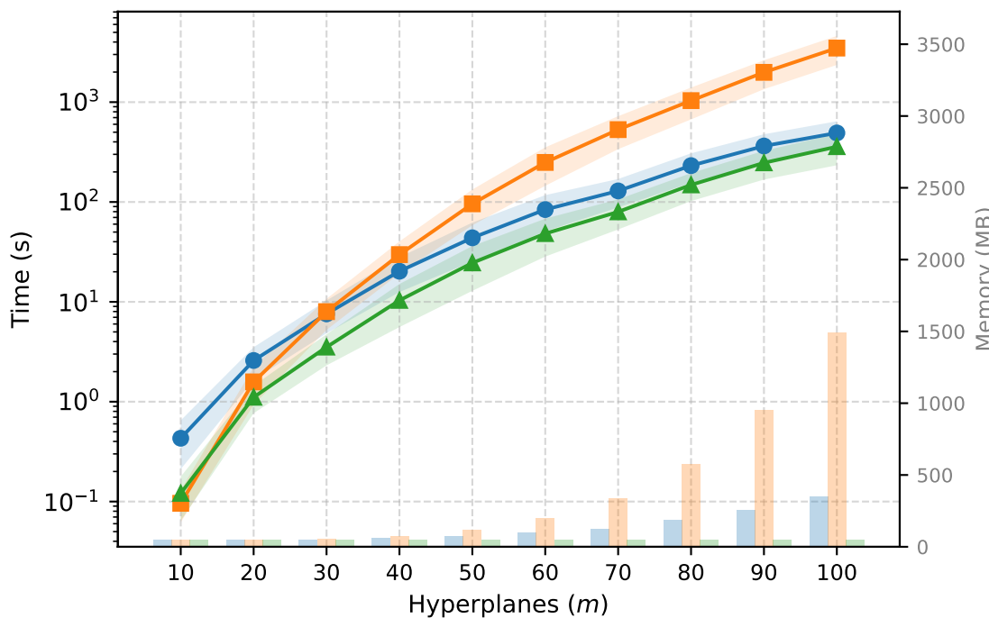
Dimension d = 4 (Runs=10)
