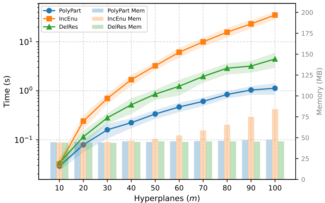
Dimension d = 2 (Runs=10)
