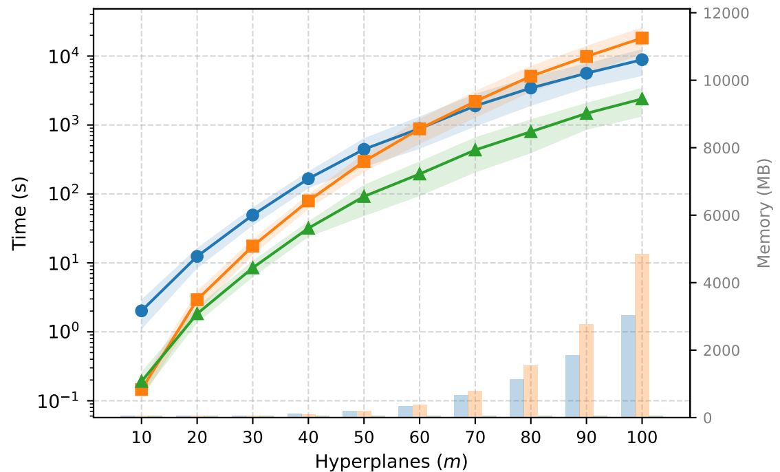
Dimension d = 5 (Runs=10)
