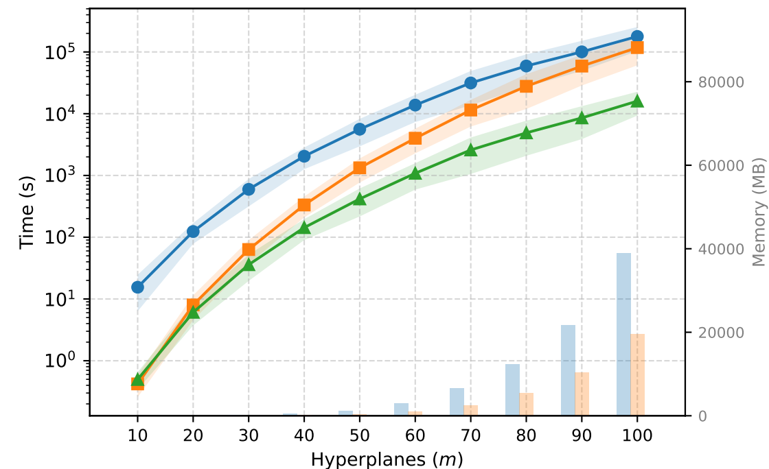
Dimension d = 6 (Runs=10)
