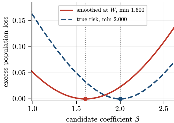
(a) smoothing moves the minimiser to \bar{\beta}
