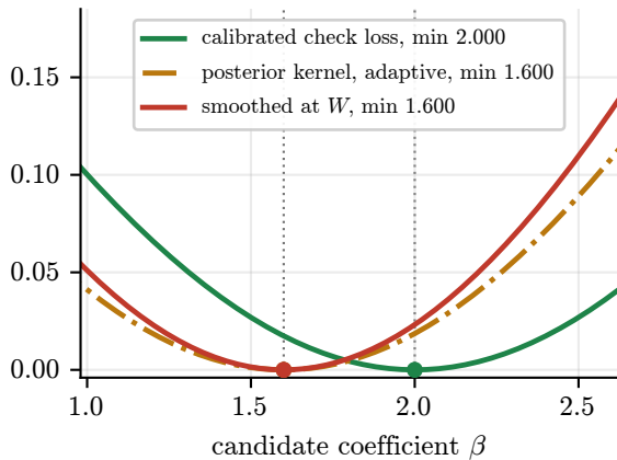
(b) conditioning keeps it at \beta^*
