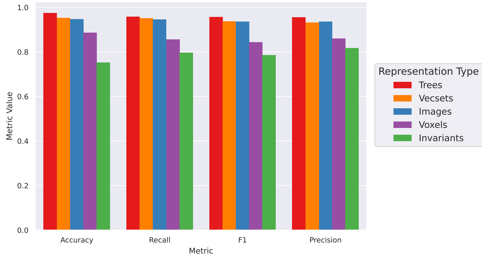
Classification Metrics (Macro Averaged)
