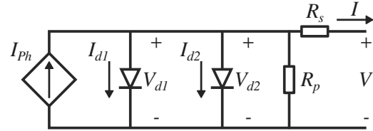
Figure 0.5: Two diode R_s and R_p PV cell model
