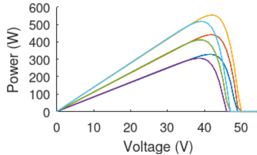
Figure 6.3: Power-voltage plot of the example module
