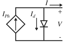
Figure 0.2: One diode ideal cell model
