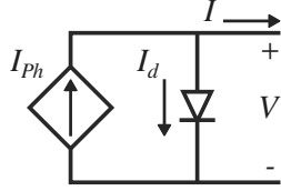
Figure 1.1: One diode ideal PV cell model
