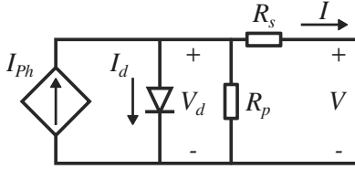
Figure 4.1: One diode R_s and R_p PV cell model
