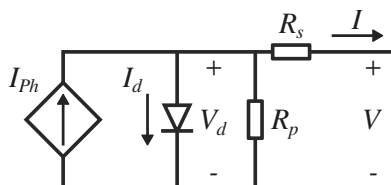
Figure 7.1: One diode R_s and R_p PV cell model
