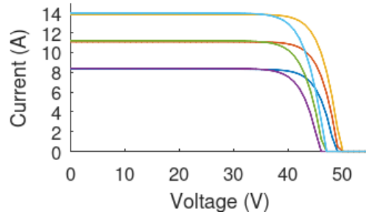
Figure 6.2: Current-voltage plot of the example module
