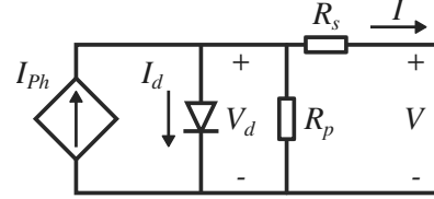
Figure 0.4: One diode R_s and R_p PV cell model
