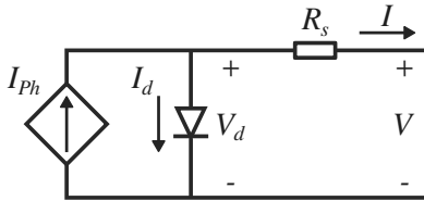
Figure 0.3: One diode R_s PV cell model
