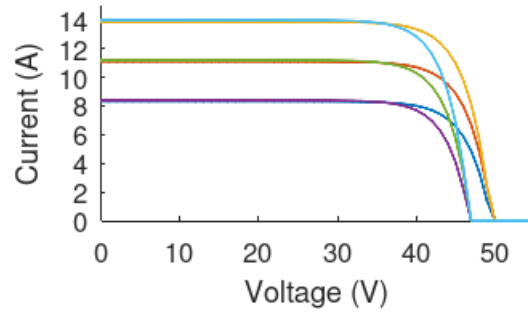
Figure 2.2: Current-voltage plot of the example module
