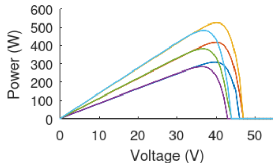
Figure 4.3: Power-voltage plot of the example module
