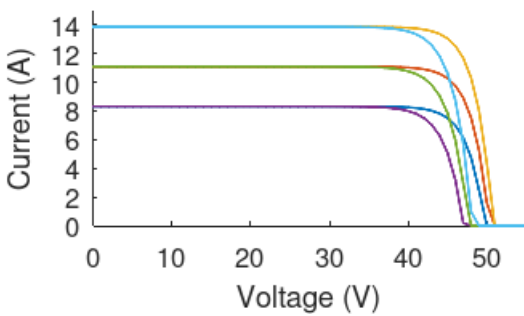
Figure 1.2: Current-voltage plot of the example module
