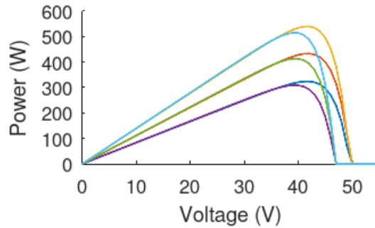
Figure 2.3: Power-voltage plot of the example module
