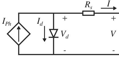
Figure 3.1: One diode R_s PV cell model
