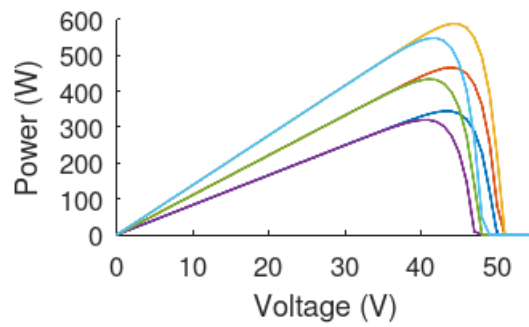
Figure 1.3: Power-voltage plot of the example module
