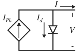
Figure 2.1: One diode ideal PV module model
