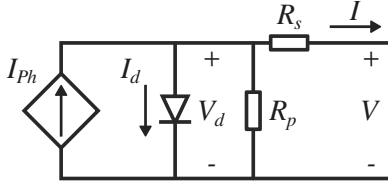
Figure 5.1: One diode with R_s and R_p PV module model
