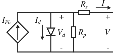
Figure 6.1: One diode R_s and R_p PV cell model
