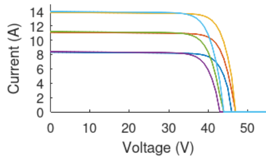
Figure 4.2: Current-voltage plot of the example module
