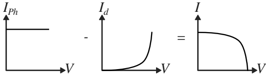
Figure 0.1: Characteristic current-voltage curve of the ideal cell model
