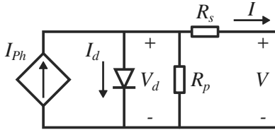
Figure 8.1: One diode R_s and R_p PV cell model
