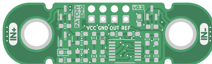
Fig. 1: PCB Front
