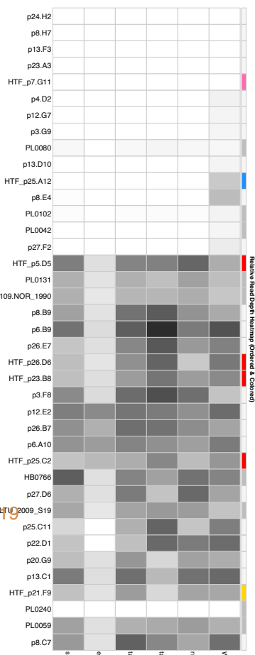
Relative Read Depth Heatmap
