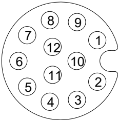
Pin arrangement
