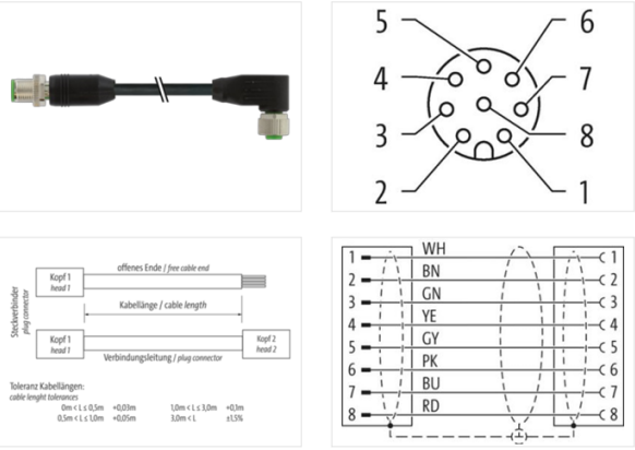
8 pin connection cable /5M 7000-48051-7170500
