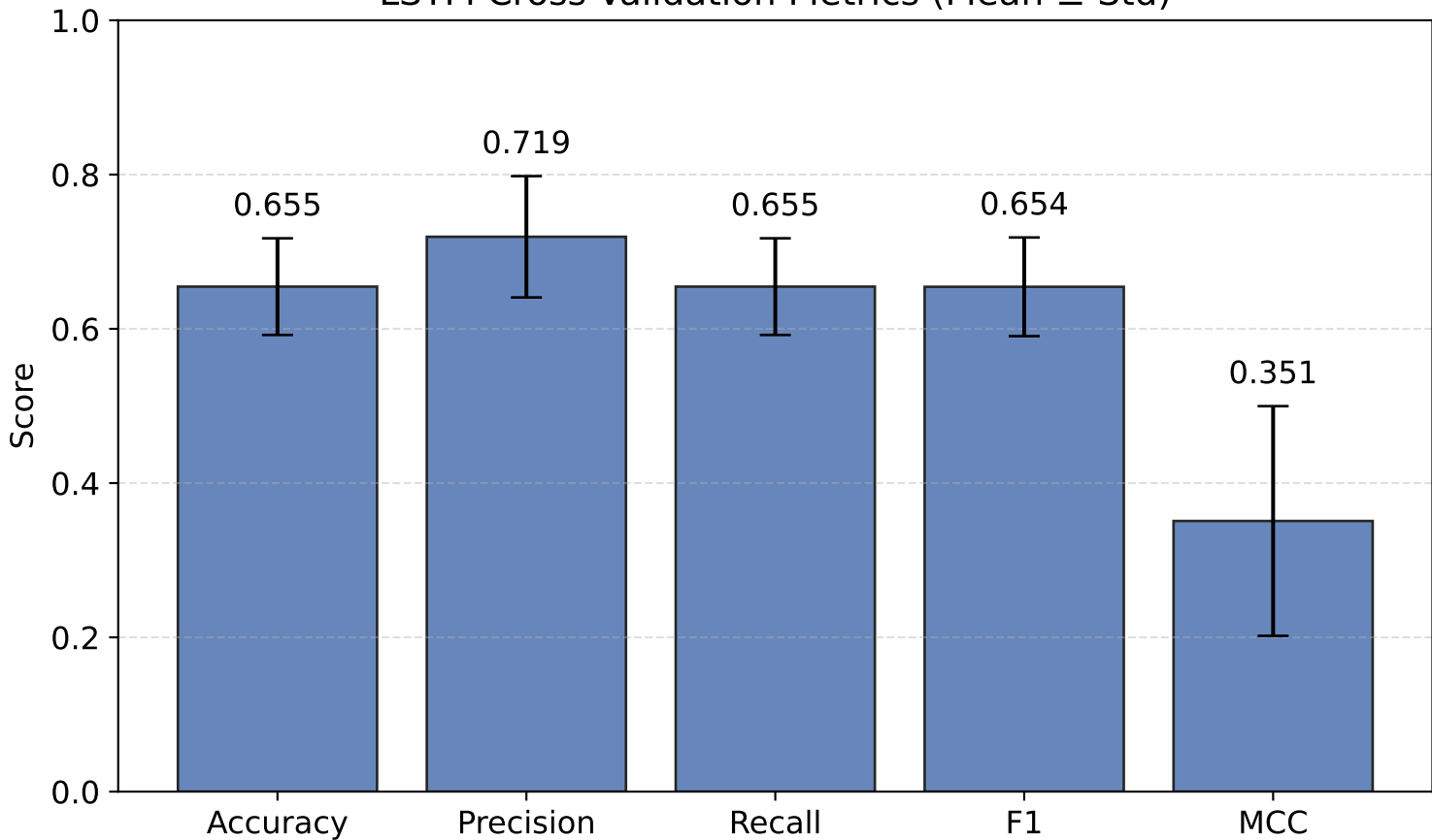
LSTM Cross-Validation Metrics (Mean \pm Std)
