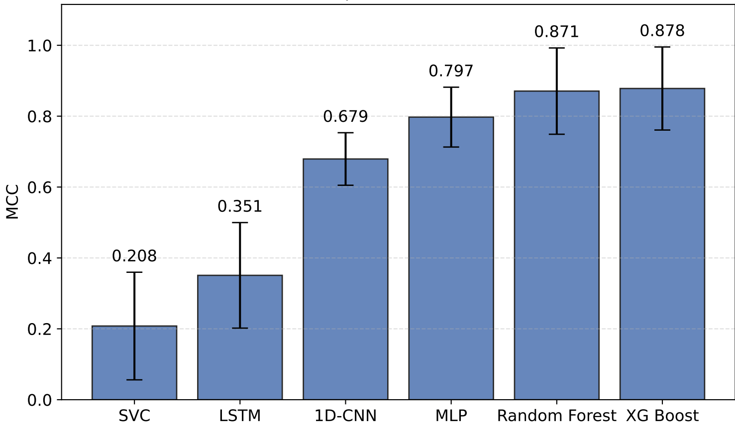
MCC Comparison (Mean \pm Std)
