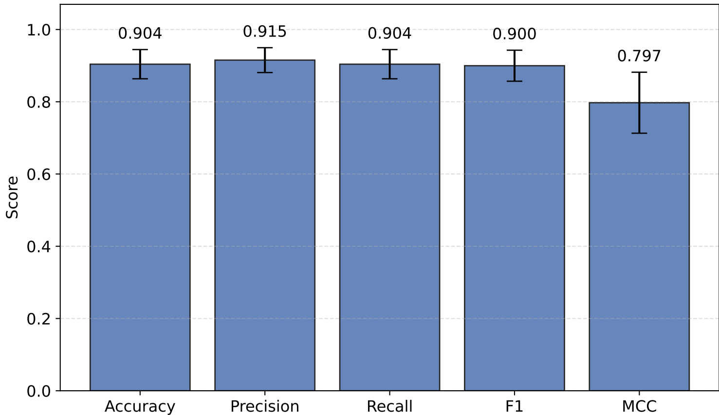
MLP Cross-Validation Metrics (Mean \pm Std)
