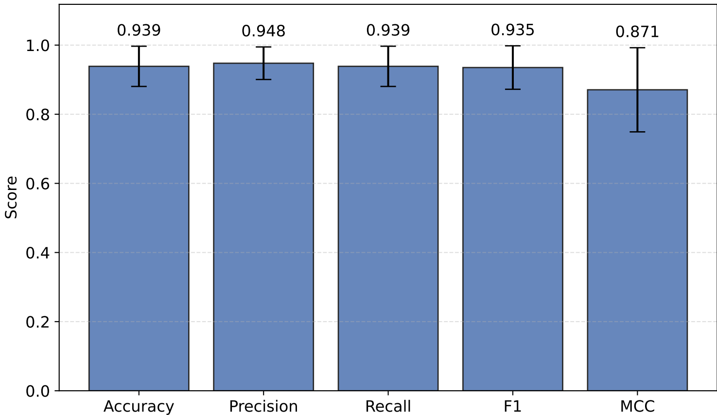
Random Forest Cross-Validation Metrics (Mean \pm Std)
