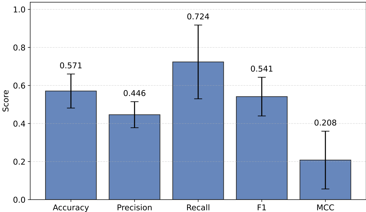
SVC Cross-Validation Metrics (Mean \pm Std)
