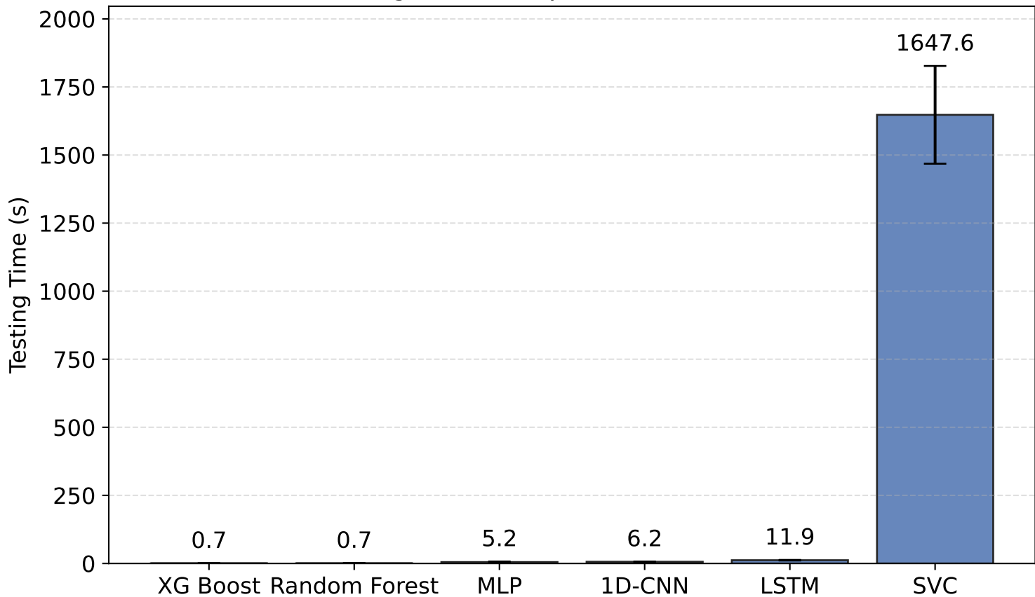
Testing Time Comparison (Mean \pm Std)
