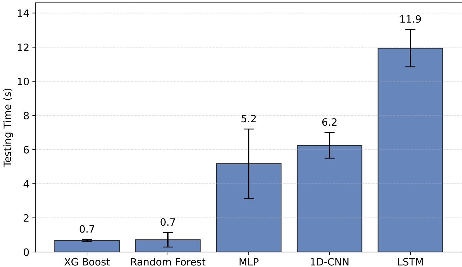
Testing Time Comparison Without SVC (Mean \pm Std)
