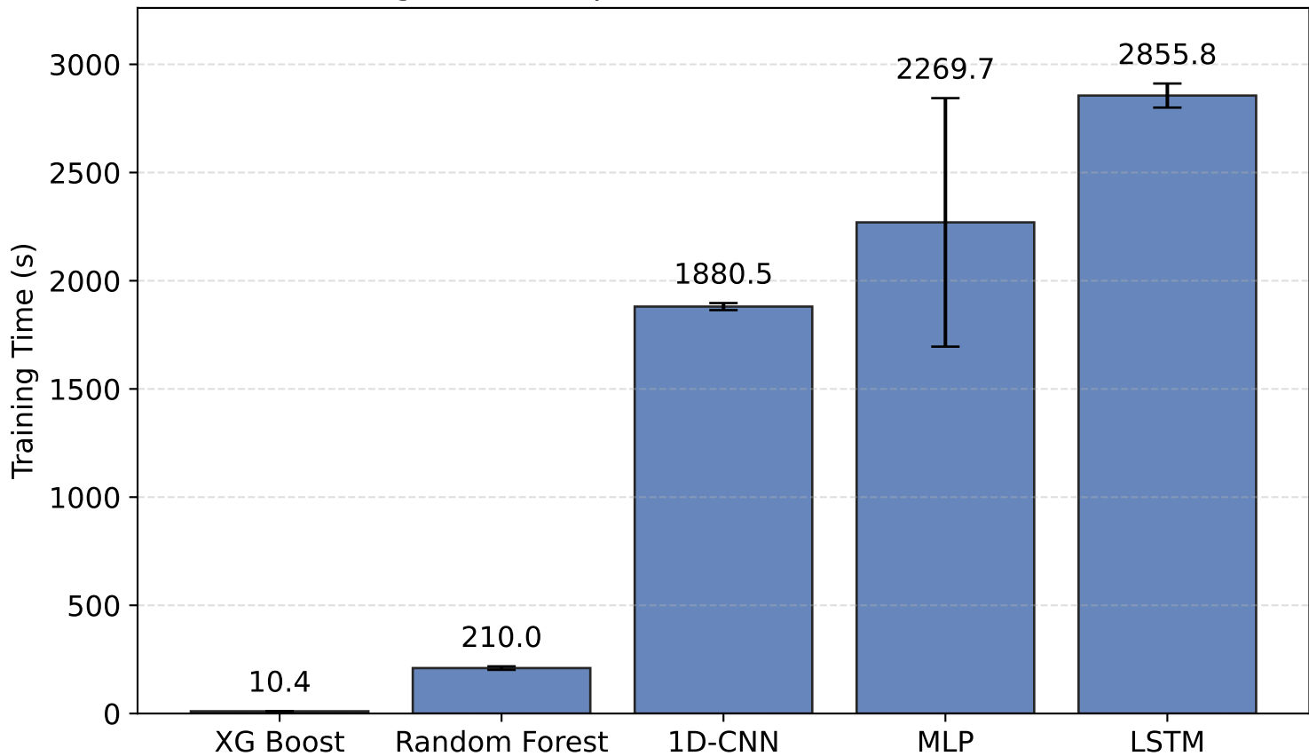
Training Time Comparison Without SVC (Mean \pm Std)
