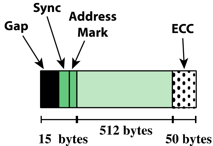
(a) Legacy 512-byte sector
