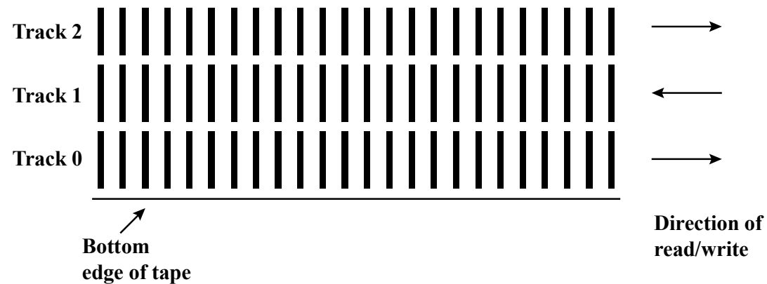
(a) Serpentine reading and writing
