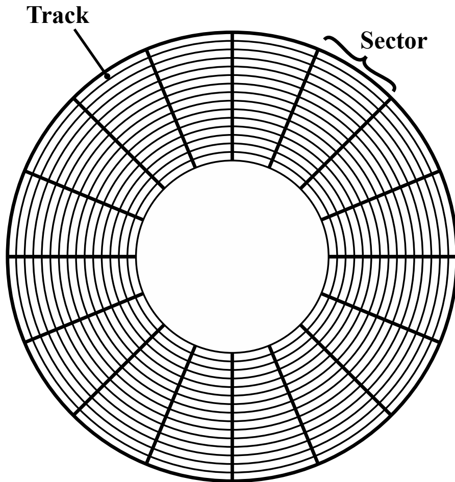
(a) Constant angular velocity
