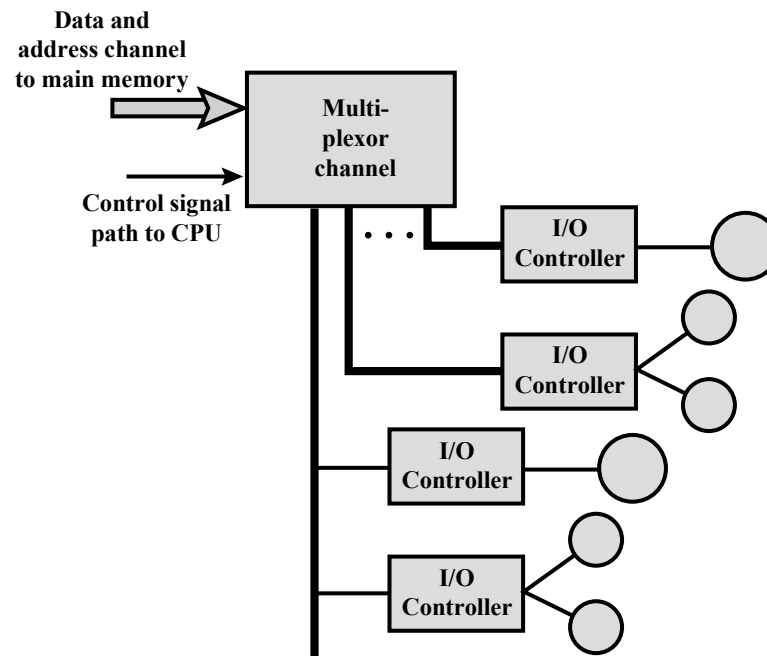
(b) Multiplexor
