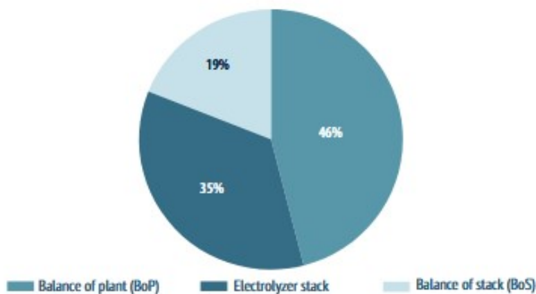
FIGURE 2.7 Breakdown of direct capital expenditure for an electrolysis system
